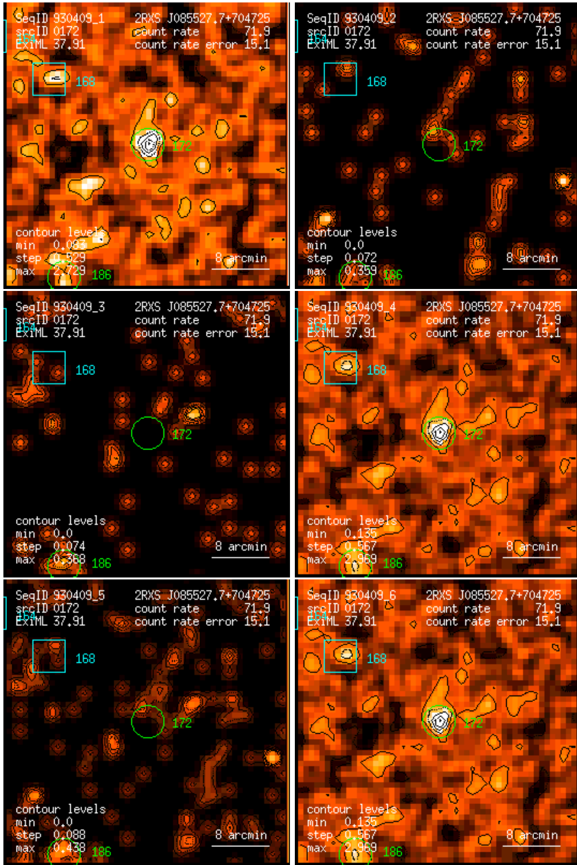
Figure 172: RASS 930409: detection 0172: band rate images, Gaussian filter: (1) PSPC channels 11 – 41, (2) 52 – 90, (3) 91 – 201, (4) 11 – 235, (5) 52 – 201, (6) 11 – 201. Broad band rates in counts/ks. Band rate contour levels in counts/ks/arcmin 2 .
