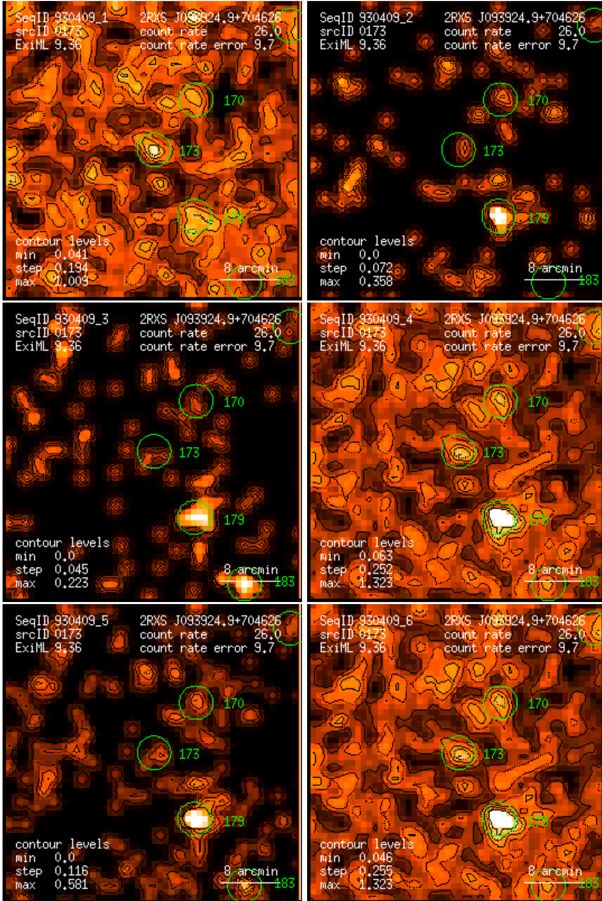
Figure 173: RASS 930409: detection 0173: band rate images, Gaussian filter: (1) PSPC channels 11 – 41, (2) 52 – 90, (3) 91 – 201, (4) 11 – 235, (5) 52 – 201, (6) 11 – 201. Broad band rates in counts/ks. Band rate contour levels in counts/ks/arcmin 2 .
