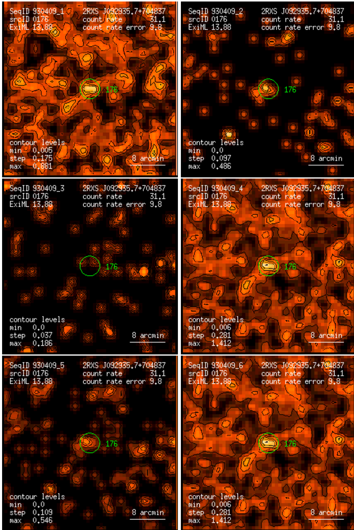
Figure 176: RASS 930409: detection 0176: band rate images, Gaussian filter: (1) PSPC channels 11 – 41, (2) 52 – 90, (3) 91 – 201, (4) 11 – 235, (5) 52 – 201, (6) 11 – 201. Broad band rates in counts/ks. Band rate contour levels in counts/ks/arcmin 2 .
