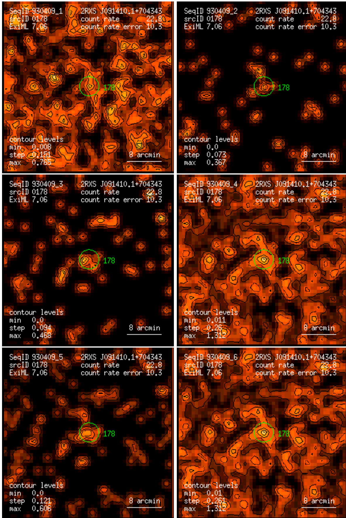
Figure 178: RASS 930409: detection 0178: band rate images, Gaussian filter: (1) PSPC channels 11 – 41, (2) 52 – 90, (3) 91 – 201, (4) 11 – 235, (5) 52 – 201, (6) 11 – 201. Broad band rates in counts/ks. Band rate contour levels in counts/ks/arcmin 2 .
