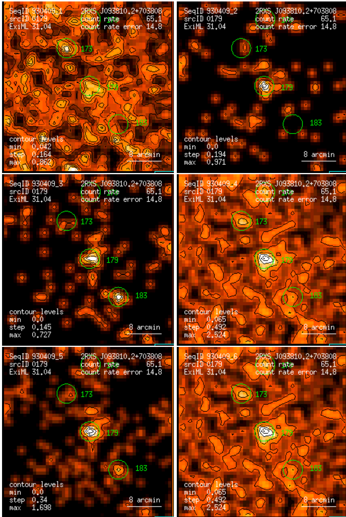
Figure 179: RASS 930409: detection 0179: band rate images, Gaussian filter: (1) PSPC channels 11 – 41, (2) 52 – 90, (3) 91 – 201, (4) 11 – 235, (5) 52 – 201, (6) 11 – 201. Broad band rates in counts/ks. Band rate contour levels in counts/ks/arcmin 2 .
