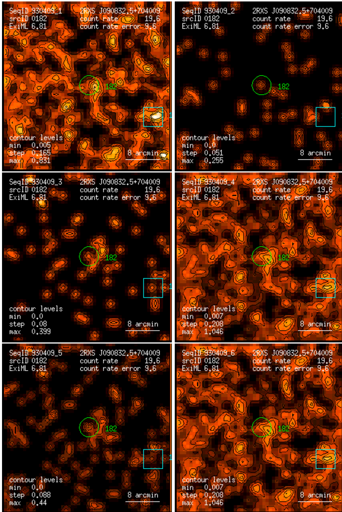
Figure 182: RASS 930409: detection 0182: band rate images, Gaussian filter: (1) PSPC channels 11 – 41, (2) 52 – 90, (3) 91 – 201, (4) 11 – 235, (5) 52 – 201, (6) 11 – 201. Broad band rates in counts/ks. Band rate contour levels in counts/ks/arcmin 2 .
