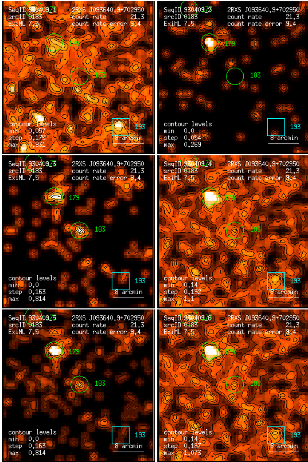
Figure 183: RASS 930409: detection 0183: band rate images, Gaussian filter: (1) PSPC channels 11 – 41, (2) 52 – 90, (3) 91 – 201, (4) 11 – 235, (5) 52 – 201, (6) 11 – 201. Broad band rates in counts/ks. Band rate contour levels in counts/ks/arcmin 2 .
