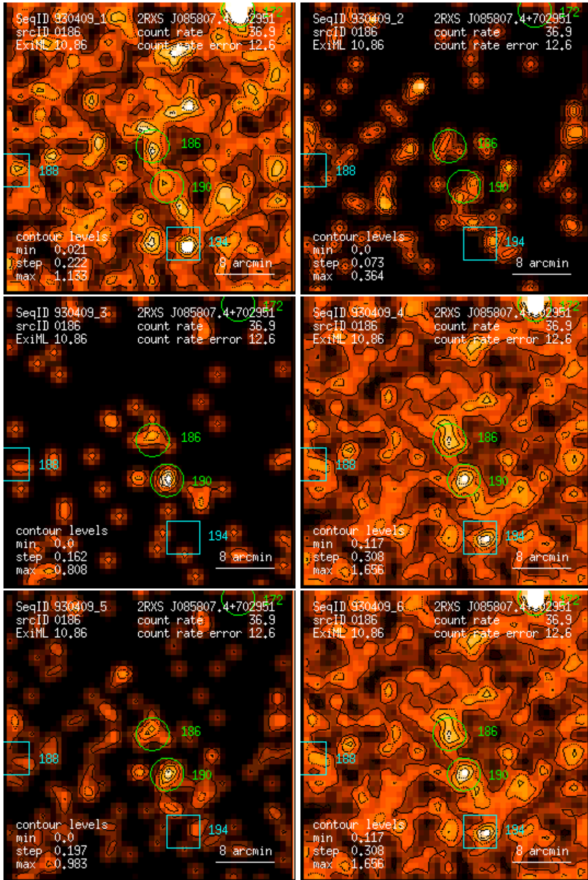
Figure 186: RASS 930409: detection 0186: band rate images, Gaussian filter: (1) PSPC channels 11 – 41, (2) 52 – 90, (3) 91 – 201, (4) 11 – 235, (5) 52 – 201, (6) 11 – 201. Broad band rates in counts/ks. Band rate contour levels in counts/ks/arcmin 2 .
