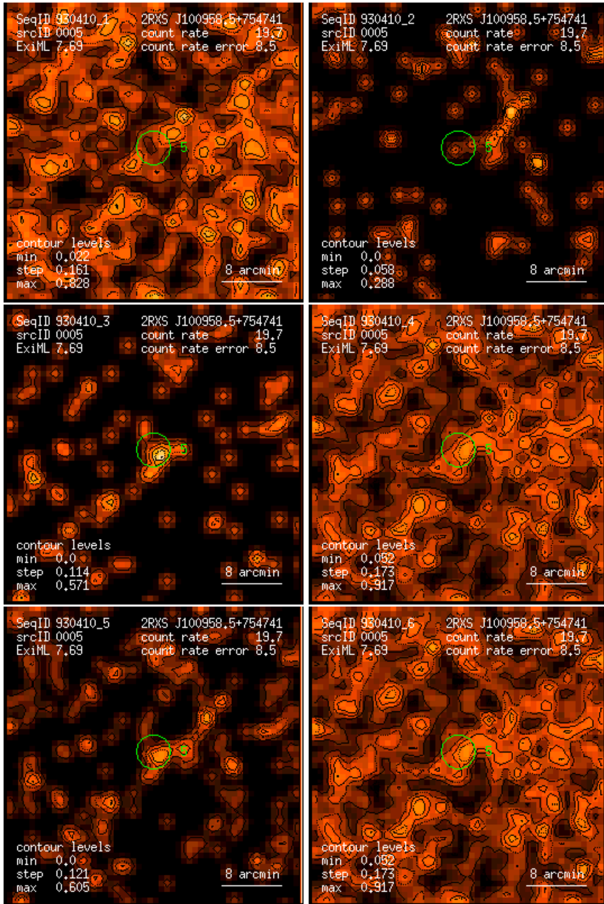
Figure 5: RASS 930410: detection 0005: band rate images, Gaussian filter: (1) PSPC channels 11 – 41, (2) 52 – 90, (3) 91 – 201, (4) 11 – 235, (5) 52 – 201, (6) 11 – 201. Broad band rates in counts/ks. Band rate contour levels in counts/ks/arcmin 2 .
