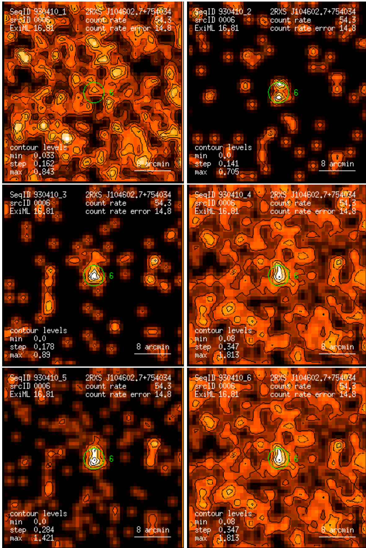
Figure 6: RASS 930410: detection 0006: band rate images, Gaussian filter: (1) PSPC channels 11 – 41, (2) 52 – 90, (3) 91 – 201, (4) 11 – 235, (5) 52 – 201, (6) 11 – 201. Broad band rates in counts/ks. Band rate contour levels in counts/ks/arcmin 2 .
