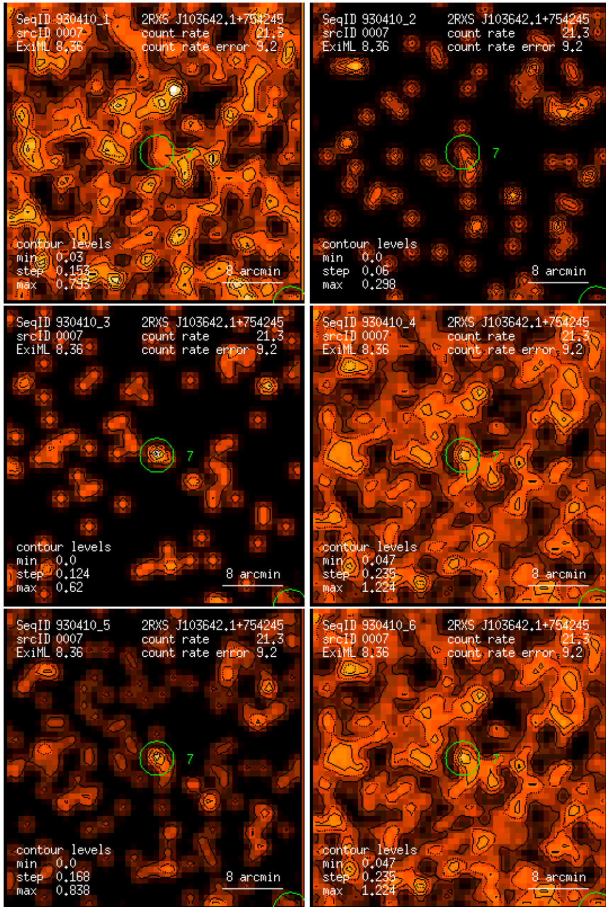
Figure 7: RASS 930410: detection 0007: band rate images, Gaussian filter: (1) PSPC channels 11 – 41, (2) 52 – 90, (3) 91 – 201, (4) 11 – 235, (5) 52 – 201, (6) 11 – 201. Broad band rates in counts/ks. Band rate contour levels in counts/ks/arcmin 2 .
