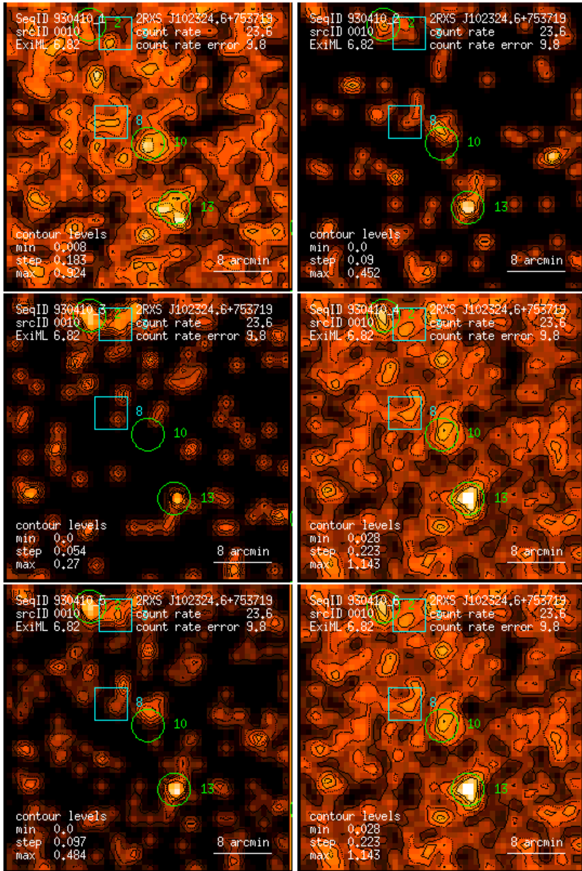
Figure 10: RASS 930410: detection 0010: band rate images, Gaussian filter: (1) PSPC channels 11 – 41, (2) 52 – 90, (3) 91 – 201, (4) 11 – 235, (5) 52 – 201, (6) 11 – 201. Broad band rates in counts/ks. Band rate contour levels in counts/ks/arcmin 2 .
