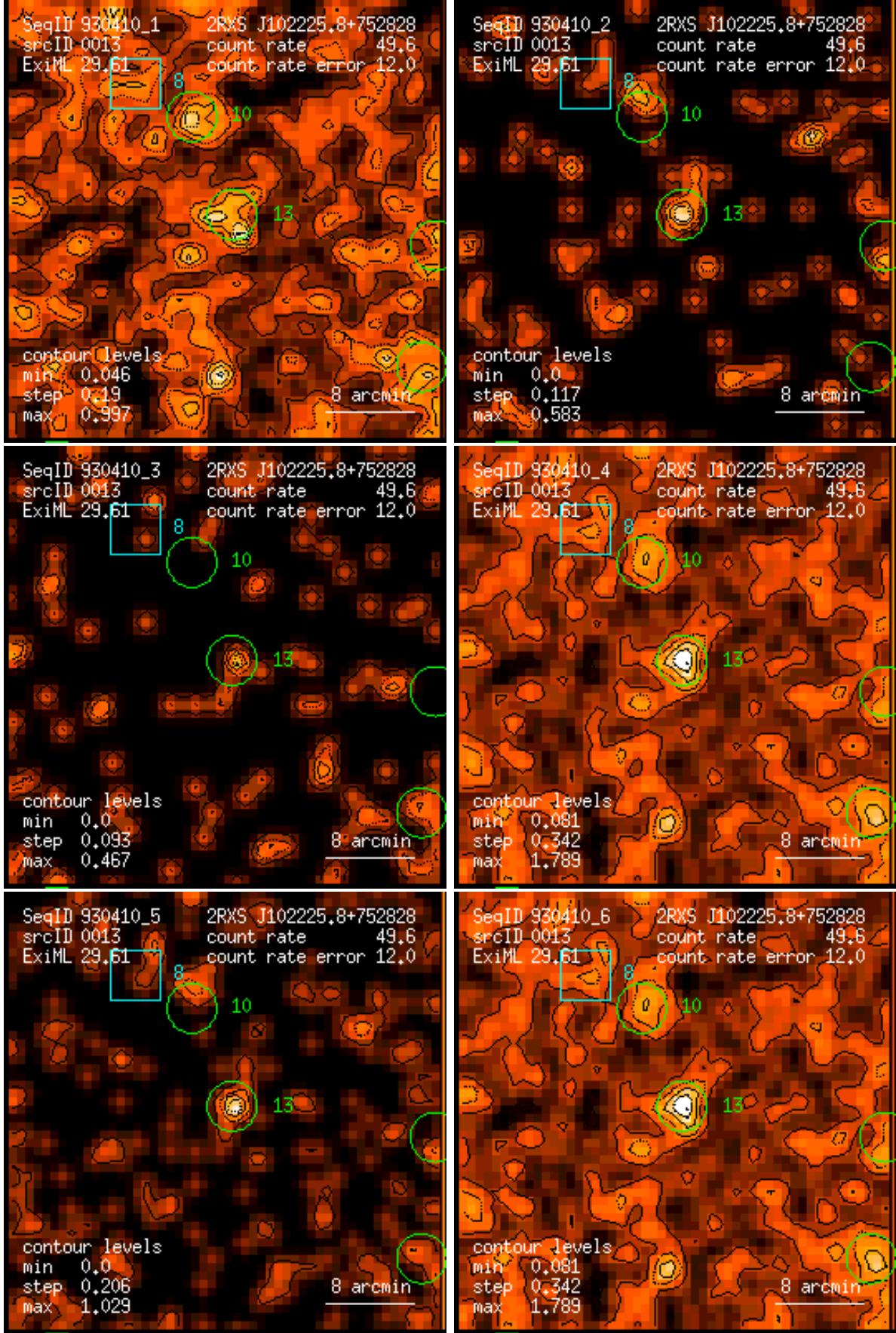
Figure 13: RASS 930410: detection 0013: band rate images, Gaussian filter: (1) PSPC channels 11 – 41, (2) 52 – 90, (3) 91 – 201, (4) 11 – 235, (5) 52 – 201, (6) 11 – 201. Broad band rates in counts/ks. Band rate contour levels in counts/ks/arcmin 2 .
