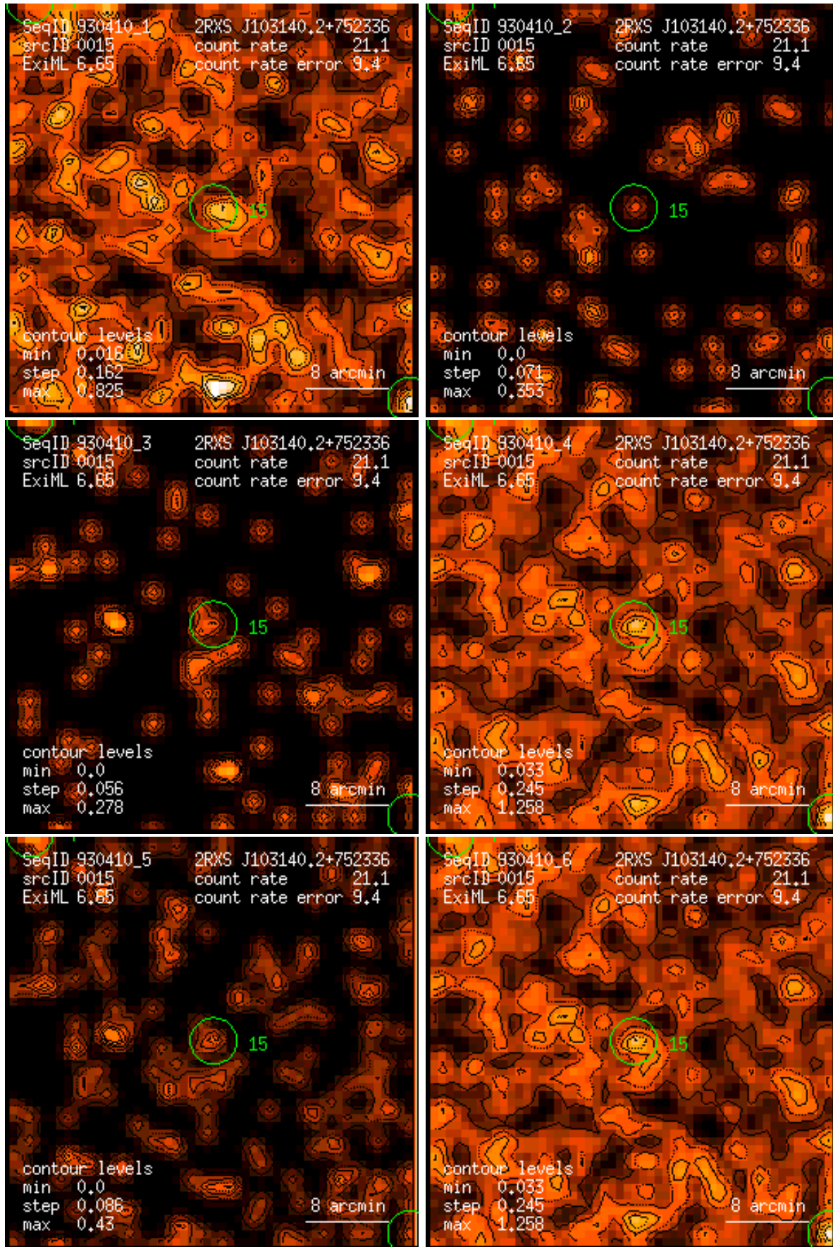
Figure 15: RASS 930410: detection 0015: band rate images, Gaussian filter: (1) PSPC channels 11 – 41, (2) 52 – 90, (3) 91 – 201, (4) 11 – 235, (5) 52 – 201, (6) 11 – 201. Broad band rates in counts/ks. Band rate contour levels in counts/ks/arcmin 2 .
