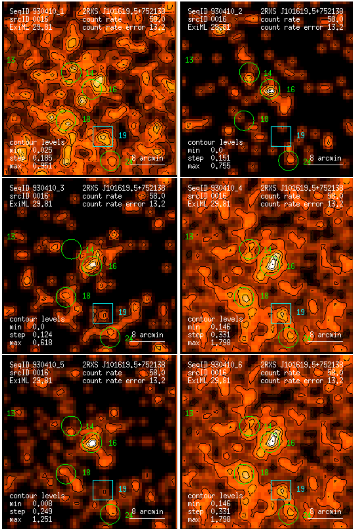
Figure 16: RASS 930410: detection 0016: band rate images, Gaussian filter: (1) PSPC channels 11 – 41, (2) 52 – 90, (3) 91 – 201, (4) 11 – 235, (5) 52 – 201, (6) 11 – 201. Broad band rates in counts/ks. Band rate contour levels in counts/ks/arcmin 2 .
