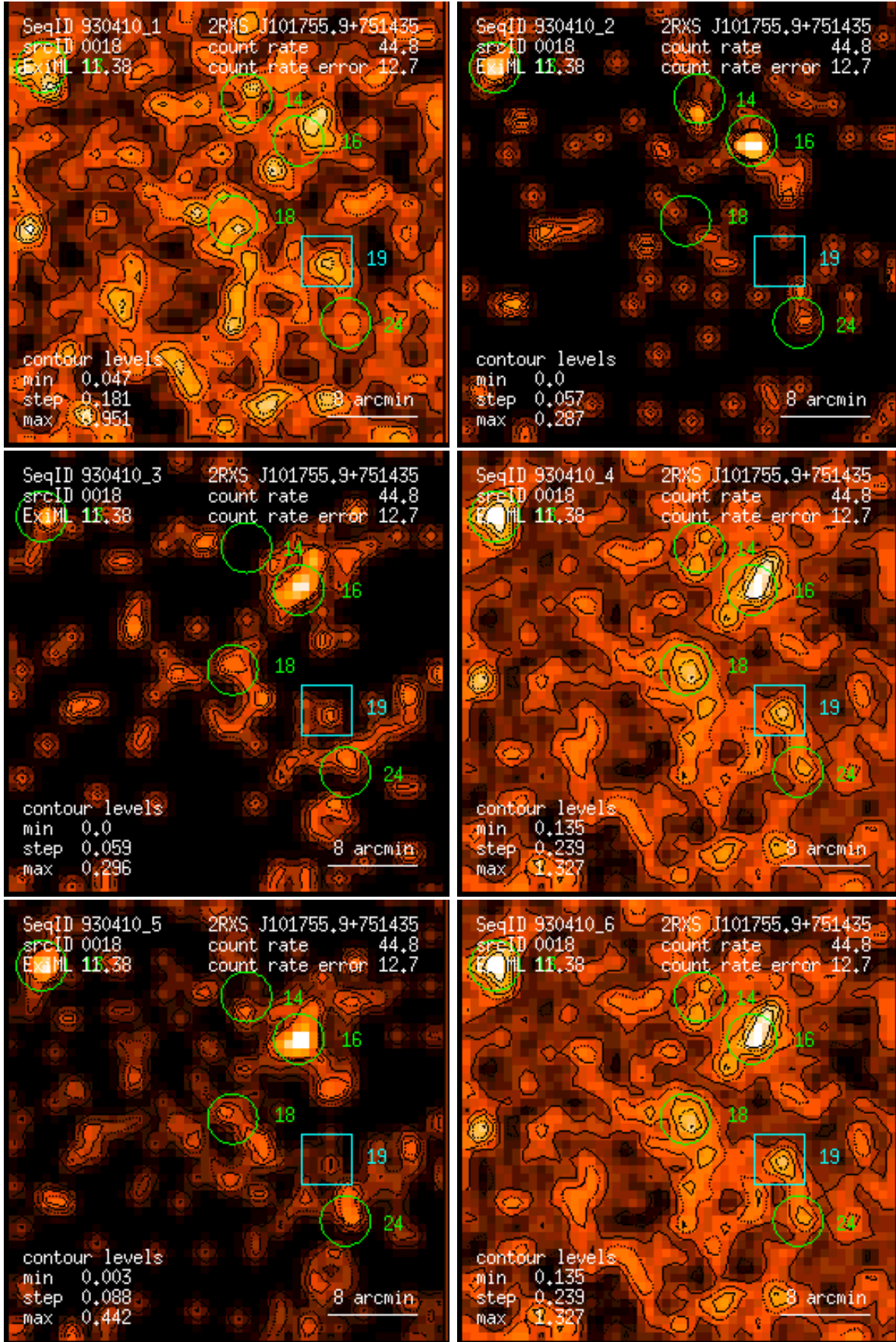
Figure 18: RASS 930410: detection 0018: band rate images, Gaussian filter: (1) PSPC channels 11 – 41, (2) 52 – 90, (3) 91 – 201, (4) 11 – 235, (5) 52 – 201, (6) 11 – 201. Broad band rates in counts/ks. Band rate contour levels in counts/ks/arcmin 2 .
