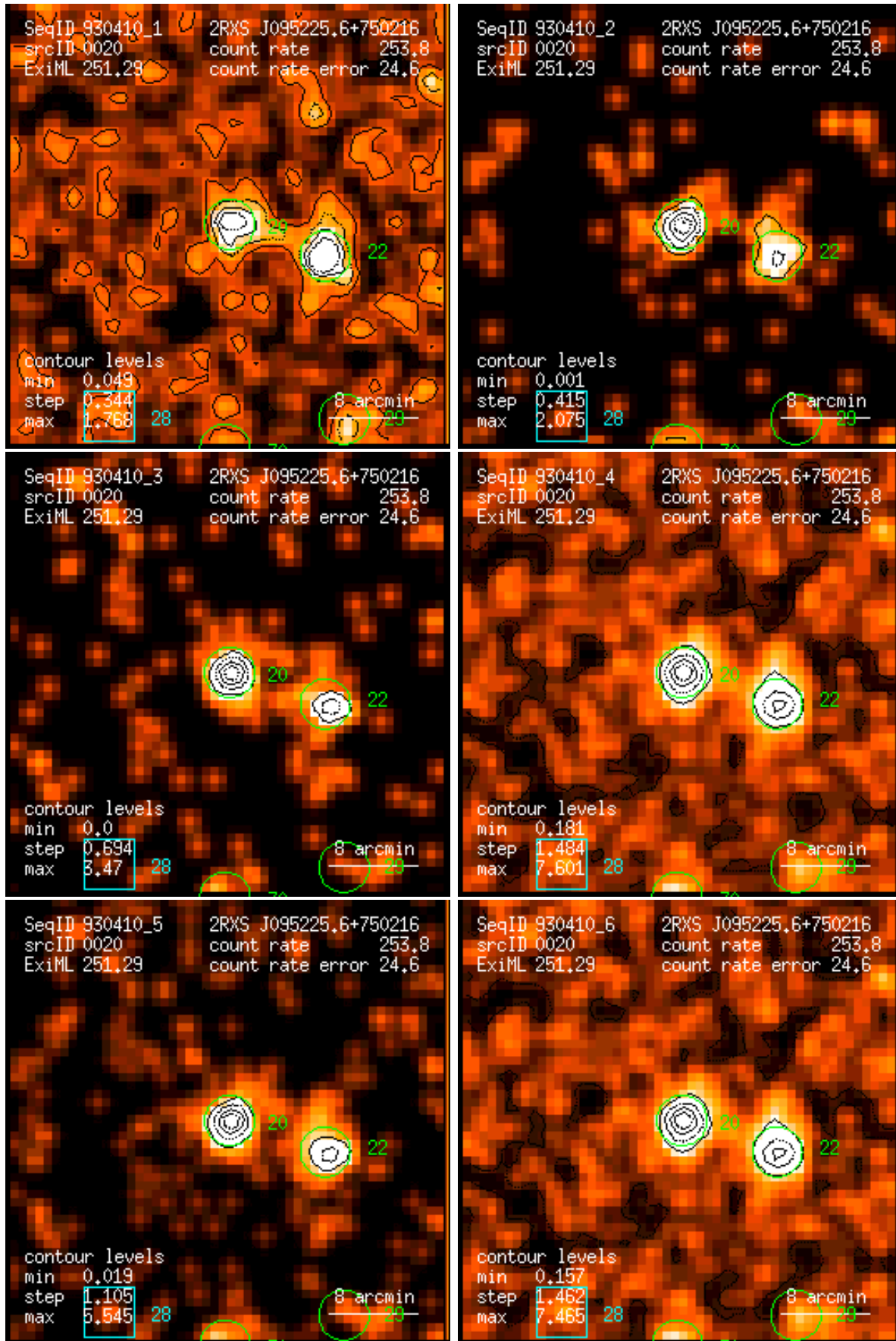
Figure 20: RASS 930410: detection 0020: band rate images, Gaussian filter: (1) PSPC channels 11 – 41, (2) 52 – 90, (3) 91 – 201, (4) 11 – 235, (5) 52 – 201, (6) 11 – 201. Broad band rates in counts/ks. Band rate contour levels in counts/ks/arcmin 2 .
