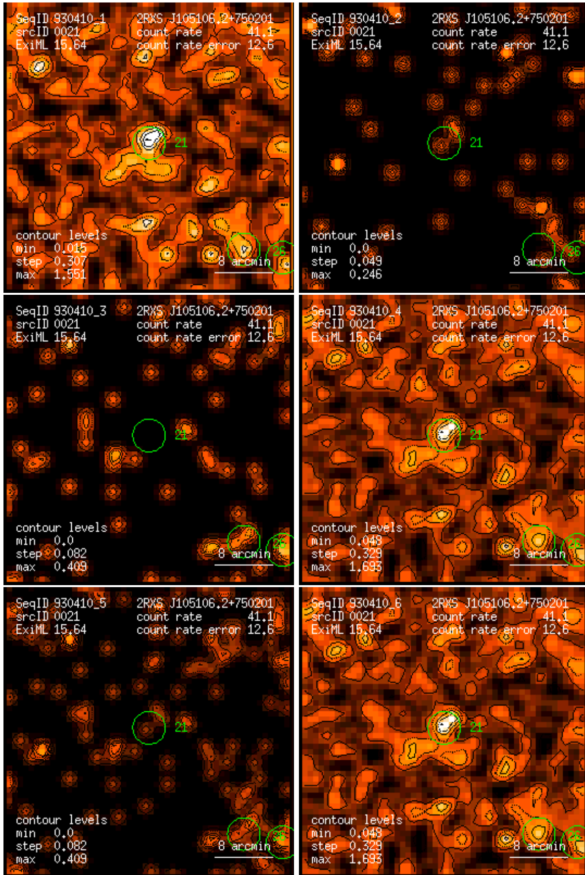
Figure 21: RASS 930410: detection 0021: band rate images, Gaussian filter: (1) PSPC channels 11 – 41, (2) 52 – 90, (3) 91 – 201, (4) 11 – 235, (5) 52 – 201, (6) 11 – 201. Broad band rates in counts/ks. Band rate contour levels in counts/ks/arcmin 2 .
