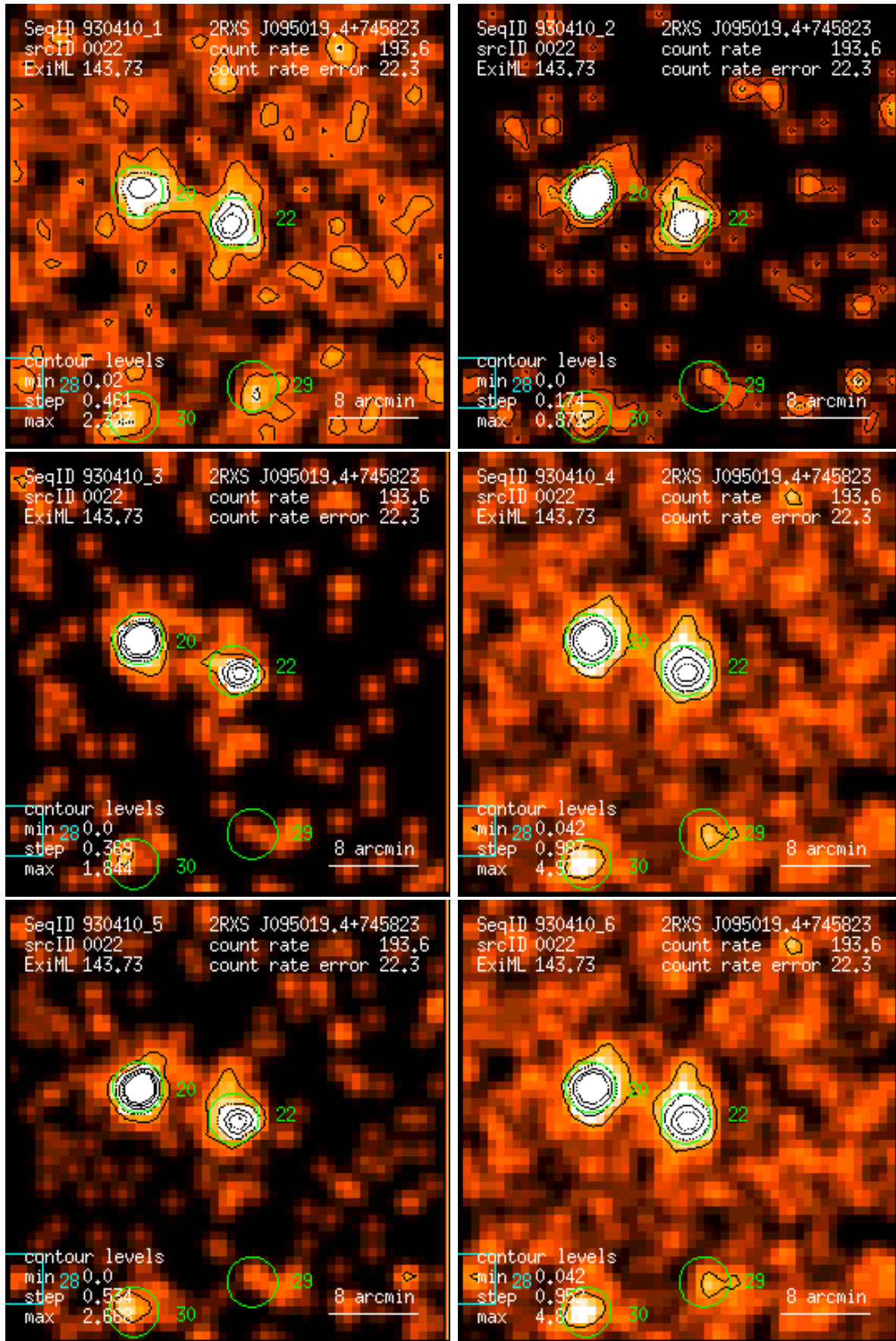
Figure 22: RASS 930410: detection 0022: band rate images, Gaussian filter: (1) PSPC channels 11 – 41, (2) 52 – 90, (3) 91 – 201, (4) 11 – 235, (5) 52 – 201, (6) 11 – 201. Broad band rates in counts/ks. Band rate contour levels in counts/ks/arcmin 2 .
