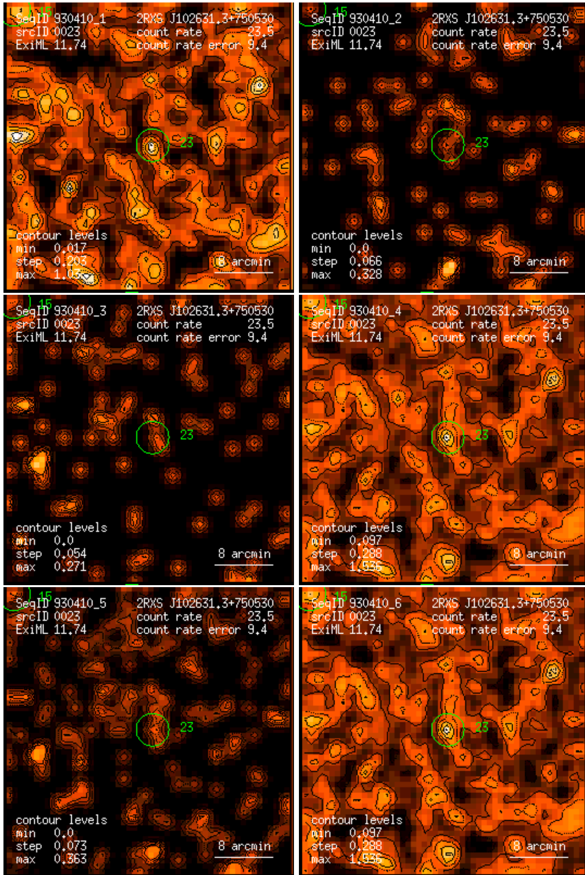
Figure 23: RASS 930410: detection 0023: band rate images, Gaussian filter: (1) PSPC channels 11 – 41, (2) 52 – 90, (3) 91 – 201, (4) 11 – 235, (5) 52 – 201, (6) 11 – 201. Broad band rates in counts/ks. Band rate contour levels in counts/ks/arcmin 2 .
