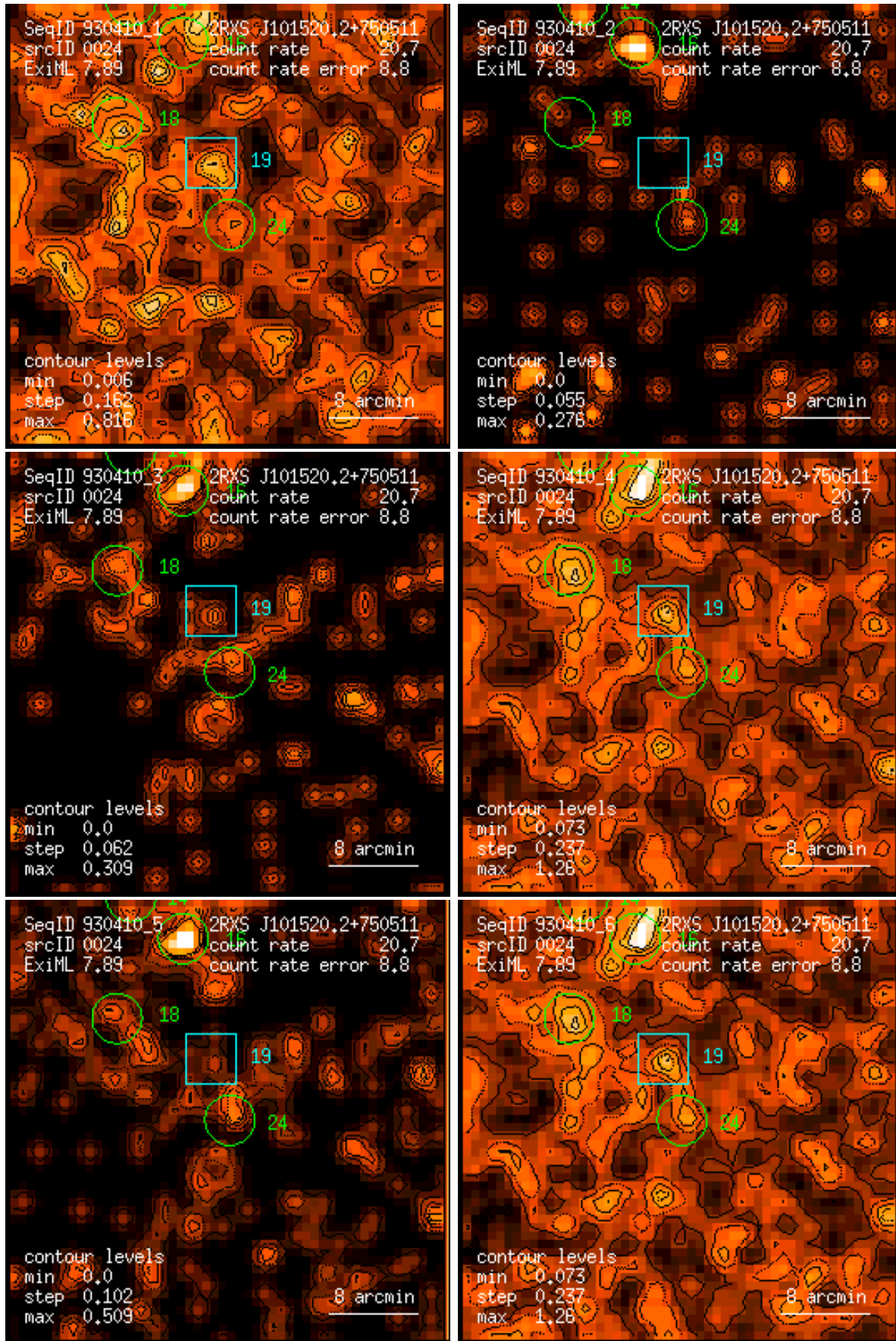
Figure 24: RASS 930410: detection 0024: band rate images, Gaussian filter: (1) PSPC channels 11 – 41, (2) 52 – 90, (3) 91 – 201, (4) 11 – 235, (5) 52 – 201, (6) 11 – 201. Broad band rates in counts/ks. Band rate contour levels in counts/ks/arcmin 2 .
