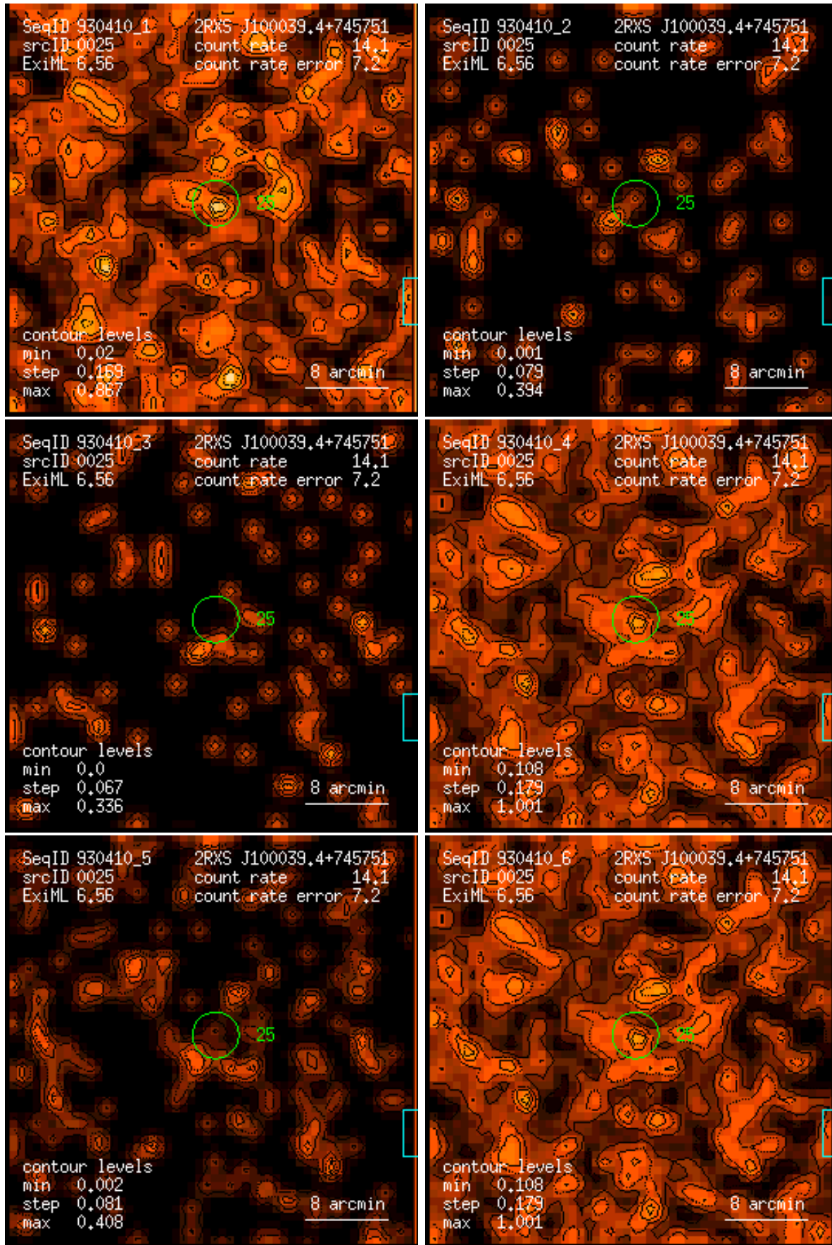
Figure 25: RASS 930410: detection 0025: band rate images, Gaussian filter: (1) PSPC channels 11 – 41, (2) 52 – 90, (3) 91 – 201, (4) 11 – 235, (5) 52 – 201, (6) 11 – 201. Broad band rates in counts/ks. Band rate contour levels in counts/ks/arcmin 2 .
