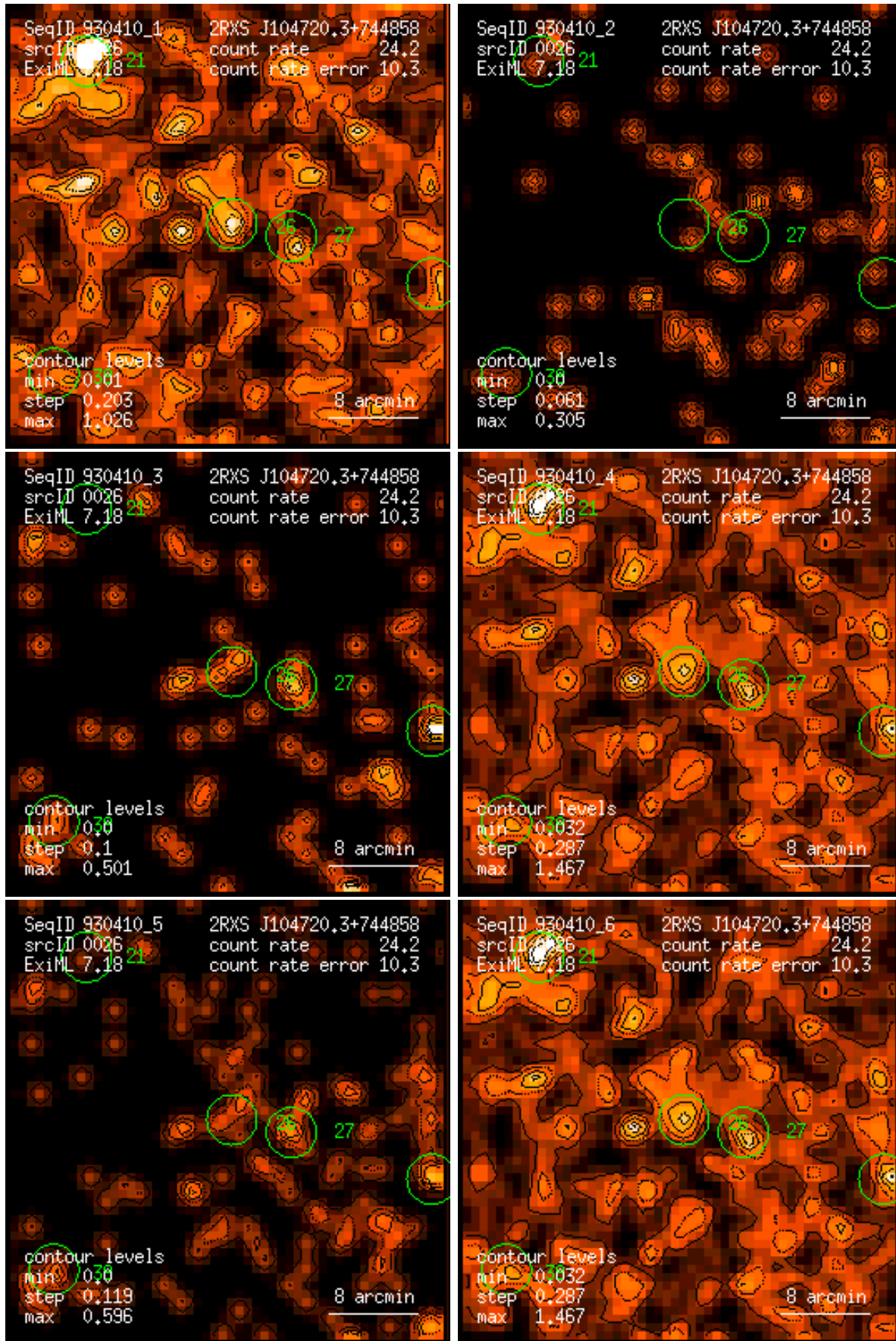
Figure 26: RASS 930410: detection 0026: band rate images, Gaussian filter: (1) PSPC channels 11 – 41, (2) 52 – 90, (3) 91 – 201, (4) 11 – 235, (5) 52 – 201, (6) 11 – 201. Broad band rates in counts/ks. Band rate contour levels in counts/ks/arcmin 2 .
