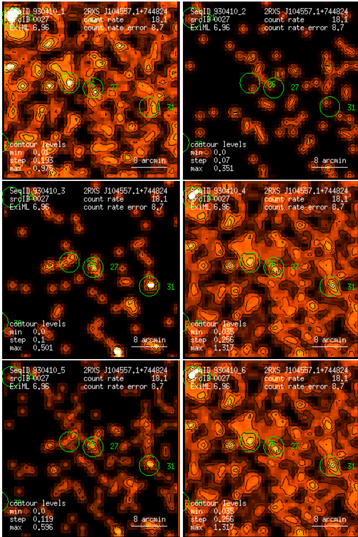
Figure 27: RASS 930410: detection 0027: band rate images, Gaussian filter: (1) PSPC channels 11 – 41, (2) 52 – 90, (3) 91 – 201, (4) 11 – 235, (5) 52 – 201, (6) 11 – 201. Broad band rates in counts/ks. Band rate contour levels in counts/ks/arcmin 2 .
