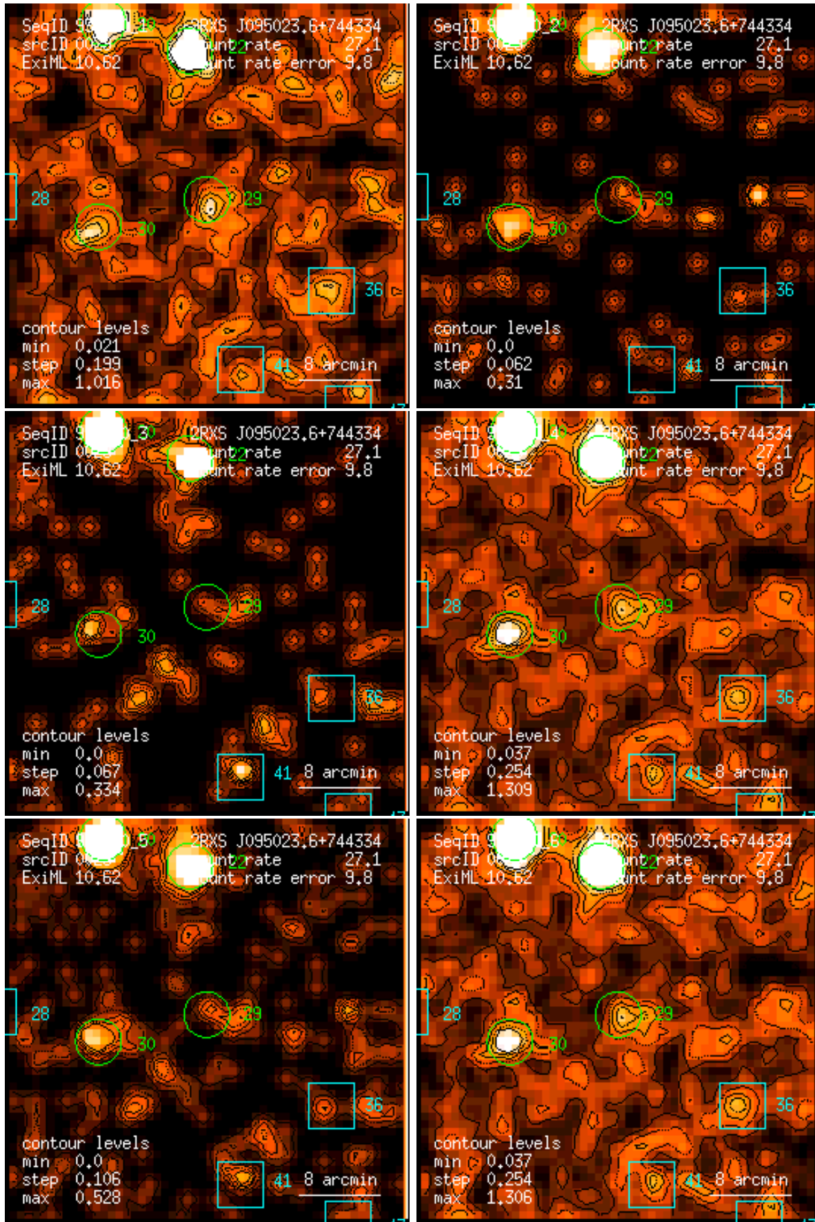
Figure 29: RASS 930410: detection 0029: band rate images, Gaussian filter: (1) PSPC channels 11 – 41, (2) 52 – 90, (3) 91 – 201, (4) 11 – 235, (5) 52 – 201, (6) 11 – 201. Broad band rates in counts/ks. Band rate contour levels in counts/ks/arcmin 2 .
