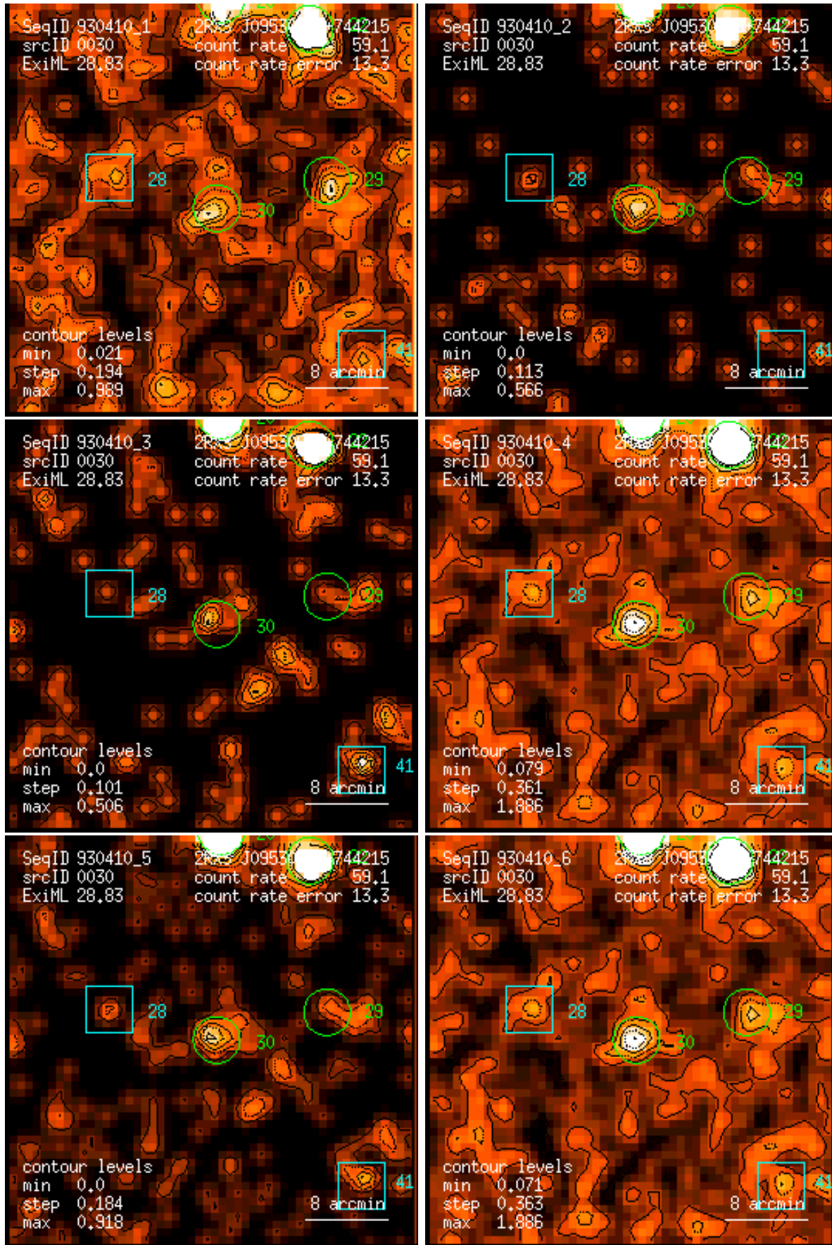
Figure 30: RASS 930410: detection 0030: band rate images, Gaussian filter: (1) PSPC channels 11 – 41, (2) 52 – 90, (3) 91 – 201, (4) 11 – 235, (5) 52 – 201, (6) 11 – 201. Broad band rates in counts/ks. Band rate contour levels in counts/ks/arcmin 2 .
