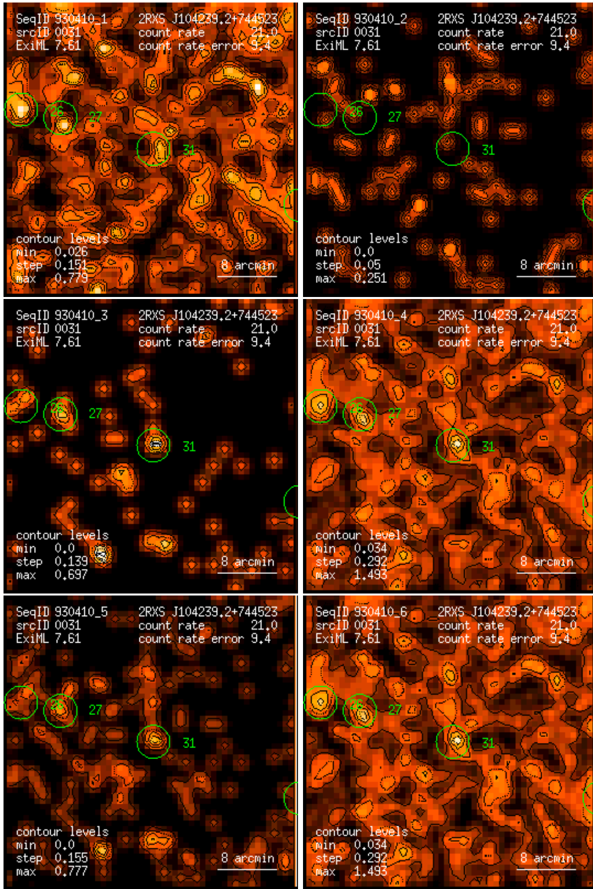
Figure 31: RASS 930410: detection 0031: band rate images, Gaussian filter: (1) PSPC channels 11 – 41, (2) 52 – 90, (3) 91 – 201, (4) 11 – 235, (5) 52 – 201, (6) 11 – 201. Broad band rates in counts/ks. Band rate contour levels in counts/ks/arcmin 2 .
