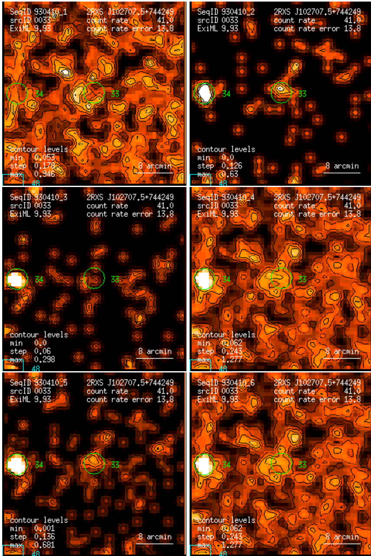
Figure 33: RASS 930410: detection 0033: band rate images, Gaussian filter: (1) PSPC channels 11 – 41, (2) 52 – 90, (3) 91 – 201, (4) 11 – 235, (5) 52 – 201, (6) 11 – 201. Broad band rates in counts/ks. Band rate contour levels in counts/ks/arcmin 2 .
