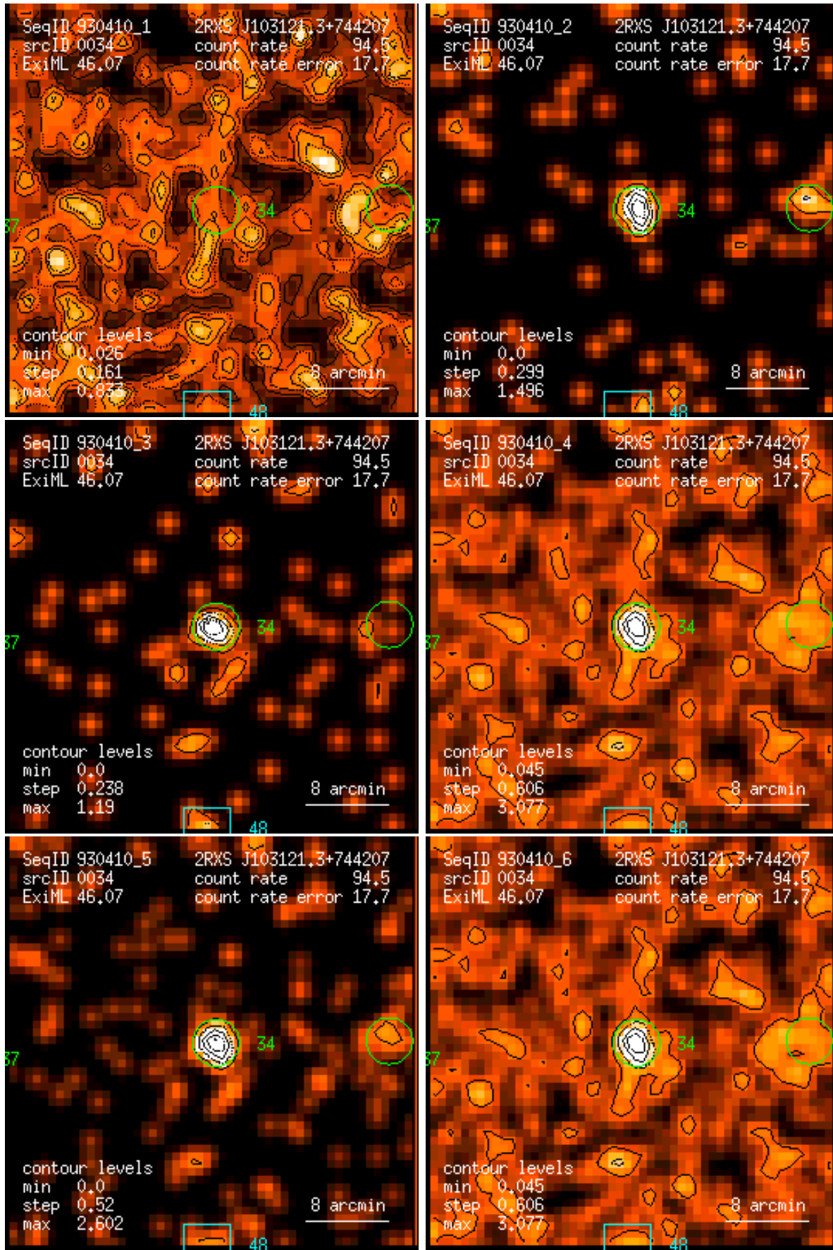
Figure 34: RASS 930410: detection 0034: band rate images, Gaussian filter: (1) PSPC channels 11 – 41, (2) 52 – 90, (3) 91 – 201, (4) 11 – 235, (5) 52 – 201, (6) 11 – 201. Broad band rates in counts/ks. Band rate contour levels in counts/ks/arcmin 2 .
