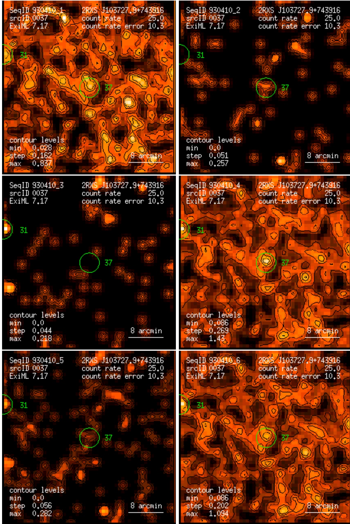
Figure 37: RASS 930410: detection 0037: band rate images, Gaussian filter: (1) PSPC channels 11 – 41, (2) 52 – 90, (3) 91 – 201, (4) 11 – 235, (5) 52 – 201, (6) 11 – 201. Broad band rates in counts/ks. Band rate contour levels in counts/ks/arcmin 2 .
