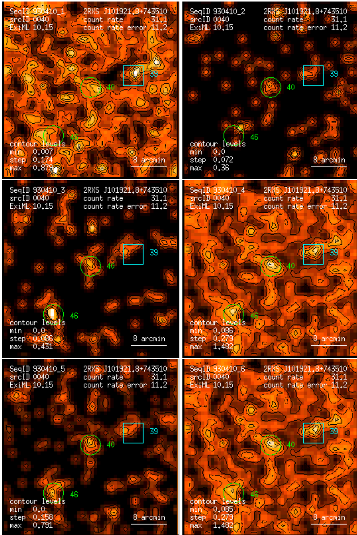
Figure 40: RASS 930410: detection 0040: band rate images, Gaussian filter: (1) PSPC channels 11 – 41, (2) 52 – 90, (3) 91 – 201, (4) 11 – 235, (5) 52 – 201, (6) 11 – 201. Broad band rates in counts/ks. Band rate contour levels in counts/ks/arcmin 2 .
