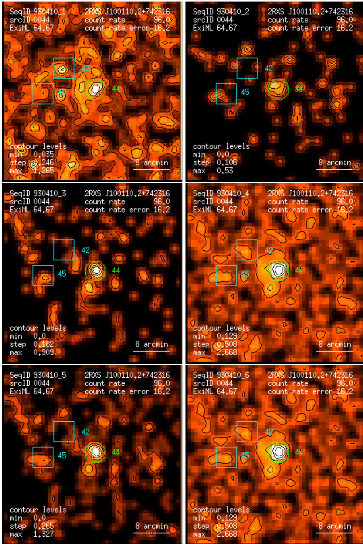
Figure 44: RASS 930410: detection 0044: band rate images, Gaussian filter: (1) PSPC channels 11 – 41, (2) 52 – 90, (3) 91 – 201, (4) 11 – 235, (5) 52 – 201, (6) 11 – 201. Broad band rates in counts/ks. Band rate contour levels in counts/ks/arcmin 2 .
