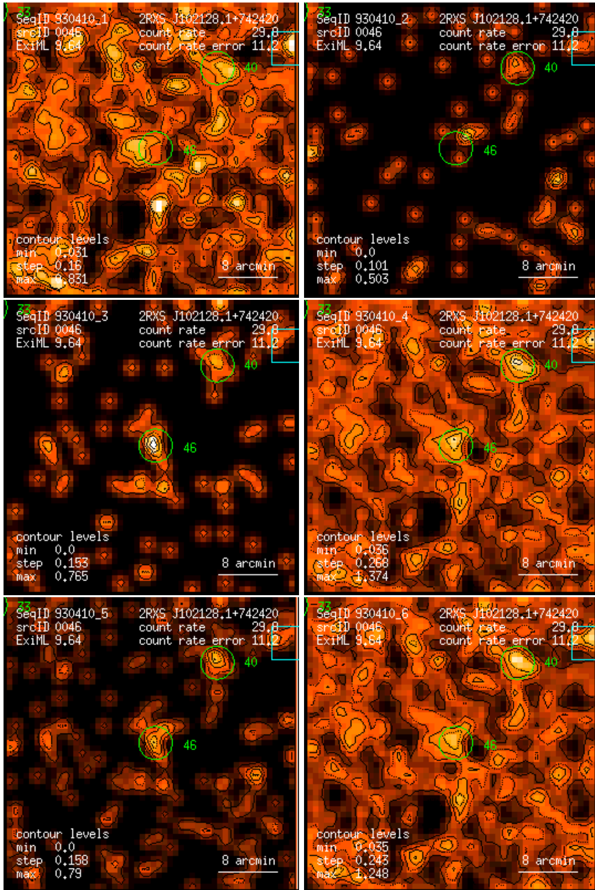
Figure 46: RASS 930410: detection 0046: band rate images, Gaussian filter: (1) PSPC channels 11 – 41, (2) 52 – 90, (3) 91 – 201, (4) 11 – 235, (5) 52 – 201, (6) 11 – 201. Broad band rates in counts/ks. Band rate contour levels in counts/ks/arcmin 2 .
