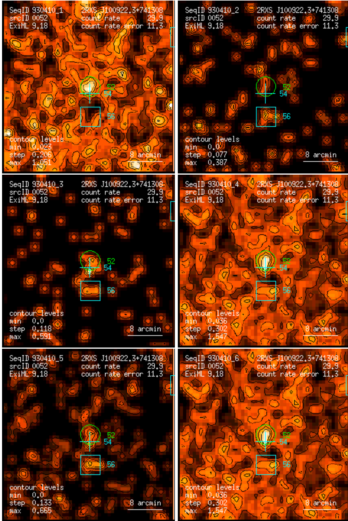
Figure 52: RASS 930410: detection 0052: band rate images, Gaussian filter: (1) PSPC channels 11 – 41, (2) 52 – 90, (3) 91 – 201, (4) 11 – 235, (5) 52 – 201, (6) 11 – 201. Broad band rates in counts/ks. Band rate contour levels in counts/ks/arcmin 2 .
