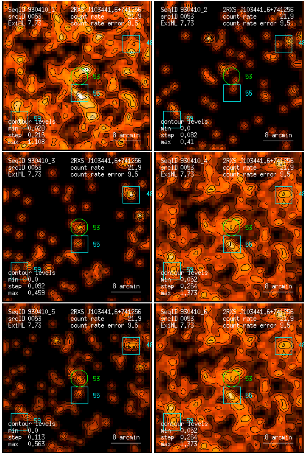
Figure 53: RASS 930410: detection 0053: band rate images, Gaussian filter: (1) PSPC channels 11 – 41, (2) 52 – 90, (3) 91 – 201, (4) 11 – 235, (5) 52 – 201, (6) 11 – 201. Broad band rates in counts/ks. Band rate contour levels in counts/ks/arcmin 2 .
