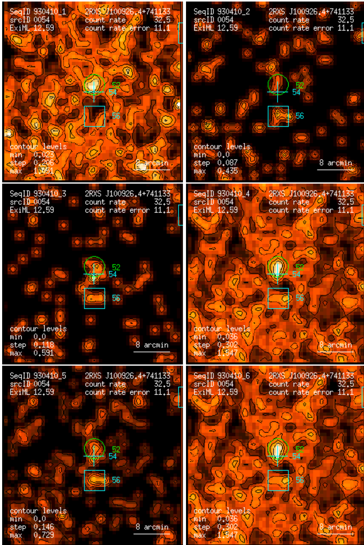
Figure 54: RASS 930410: detection 0054: band rate images, Gaussian filter: (1) PSPC channels 11 – 41, (2) 52 – 90, (3) 91 – 201, (4) 11 – 235, (5) 52 – 201, (6) 11 – 201. Broad band rates in counts/ks. Band rate contour levels in counts/ks/arcmin 2 .
