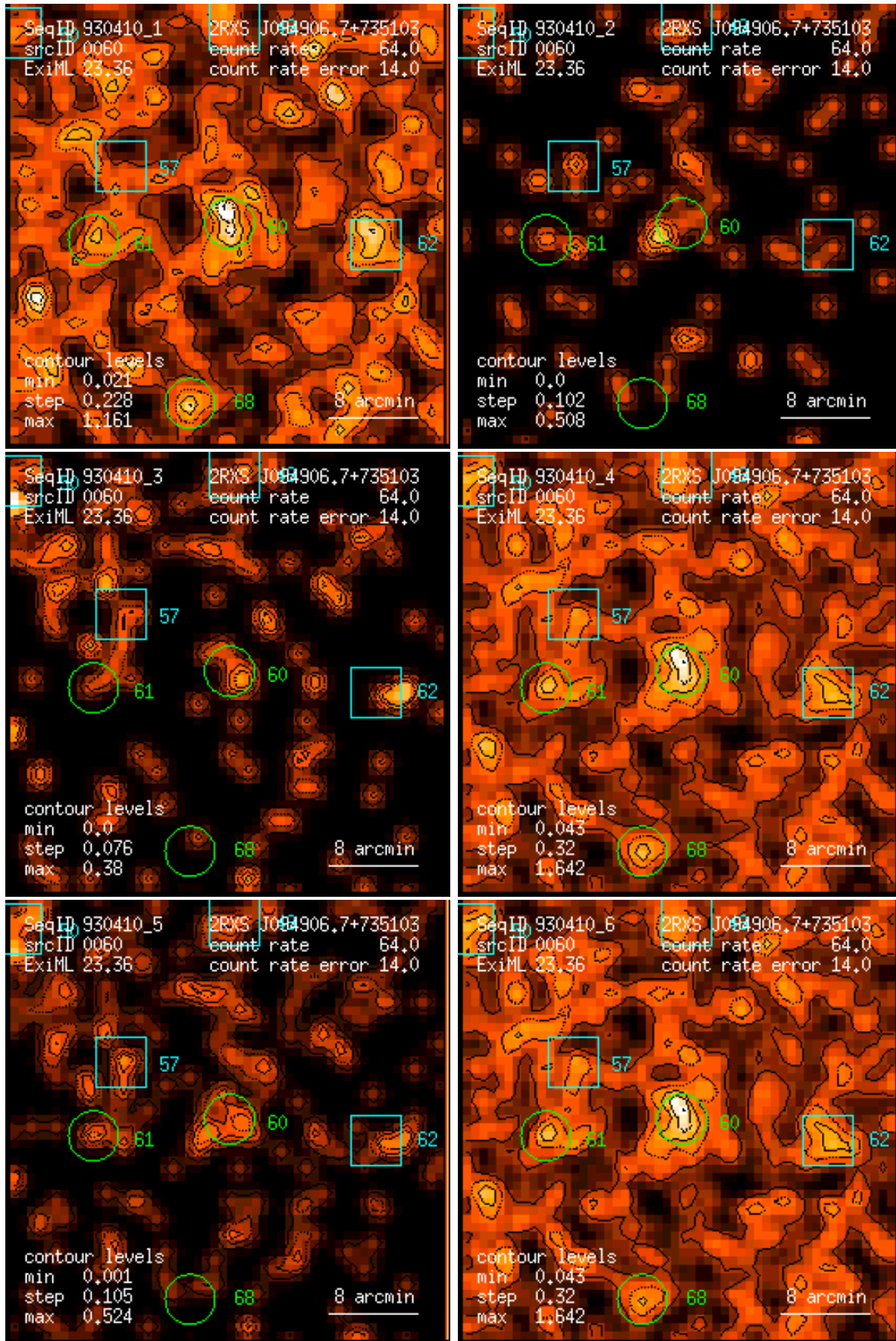
Figure 60: RASS 930410: detection 0060: band rate images, Gaussian filter: (1) PSPC channels 11 – 41, (2) 52 – 90, (3) 91 – 201, (4) 11 – 235, (5) 52 – 201, (6) 11 – 201. Broad band rates in counts/ks. Band rate contour levels in counts/ks/arcmin 2 .
