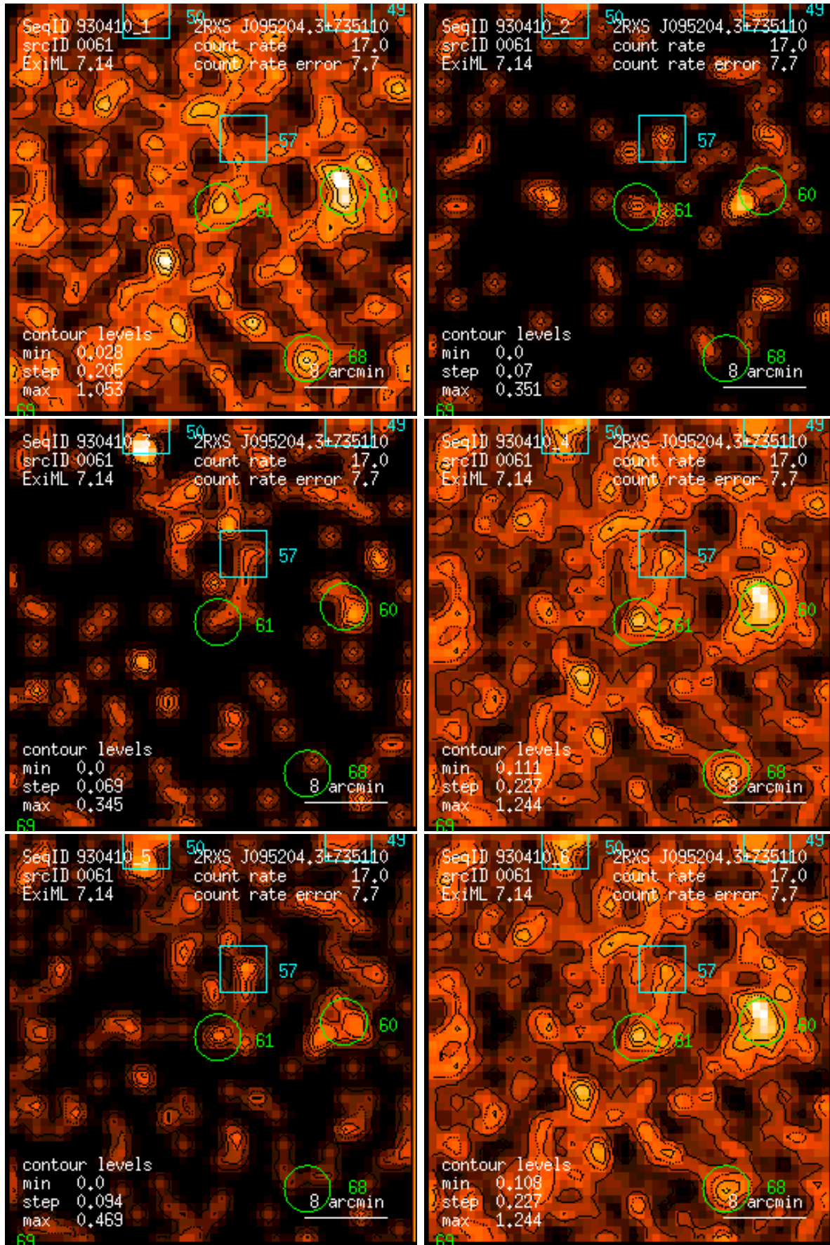
Figure 61: RASS 930410: detection 0061: band rate images, Gaussian filter: (1) PSPC channels 11 – 41, (2) 52 – 90, (3) 91 – 201, (4) 11 – 235, (5) 52 – 201, (6) 11 – 201. Broad band rates in counts/ks. Band rate contour levels in counts/ks/arcmin 2 .
