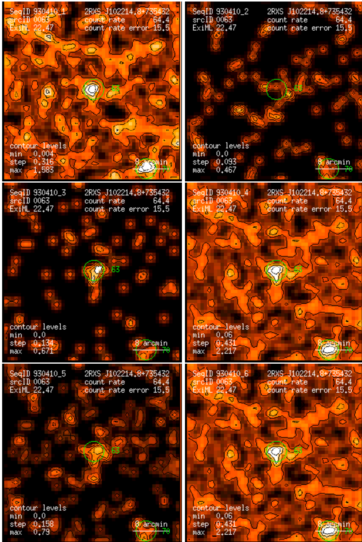
Figure 63: RASS 930410: detection 0063: band rate images, Gaussian filter: (1) PSPC channels 11 – 41, (2) 52 – 90, (3) 91 – 201, (4) 11 – 235, (5) 52 – 201, (6) 11 – 201. Broad band rates in counts/ks. Band rate contour levels in counts/ks/arcmin 2 .
