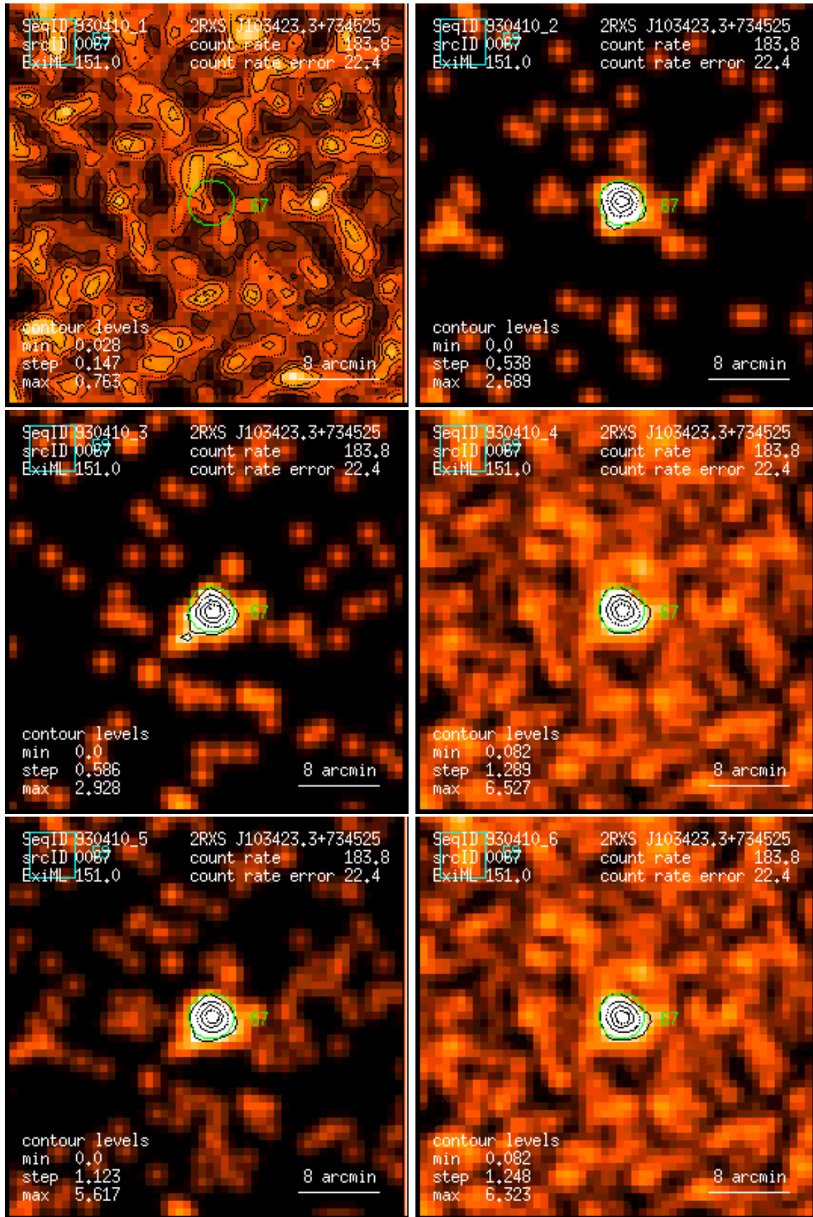
Figure 67: RASS 930410: detection 0067: band rate images, Gaussian filter: (1) PSPC channels 11 – 41, (2) 52 – 90, (3) 91 – 201, (4) 11 – 235, (5) 52 – 201, (6) 11 – 201. Broad band rates in counts/ks. Band rate contour levels in counts/ks/arcmin 2 .
