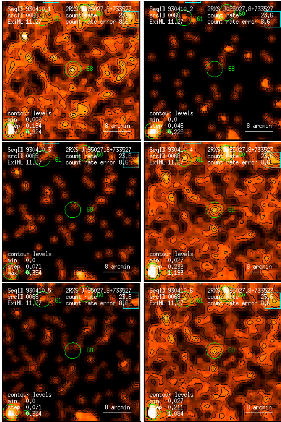
Figure 68: RASS 930410: detection 0068: band rate images, Gaussian filter: (1) PSPC channels 11 – 41, (2) 52 – 90, (3) 91 – 201, (4) 11 – 235, (5) 52 – 201, (6) 11 – 201. Broad band rates in counts/ks. Band rate contour levels in counts/ks/arcmin 2 .
