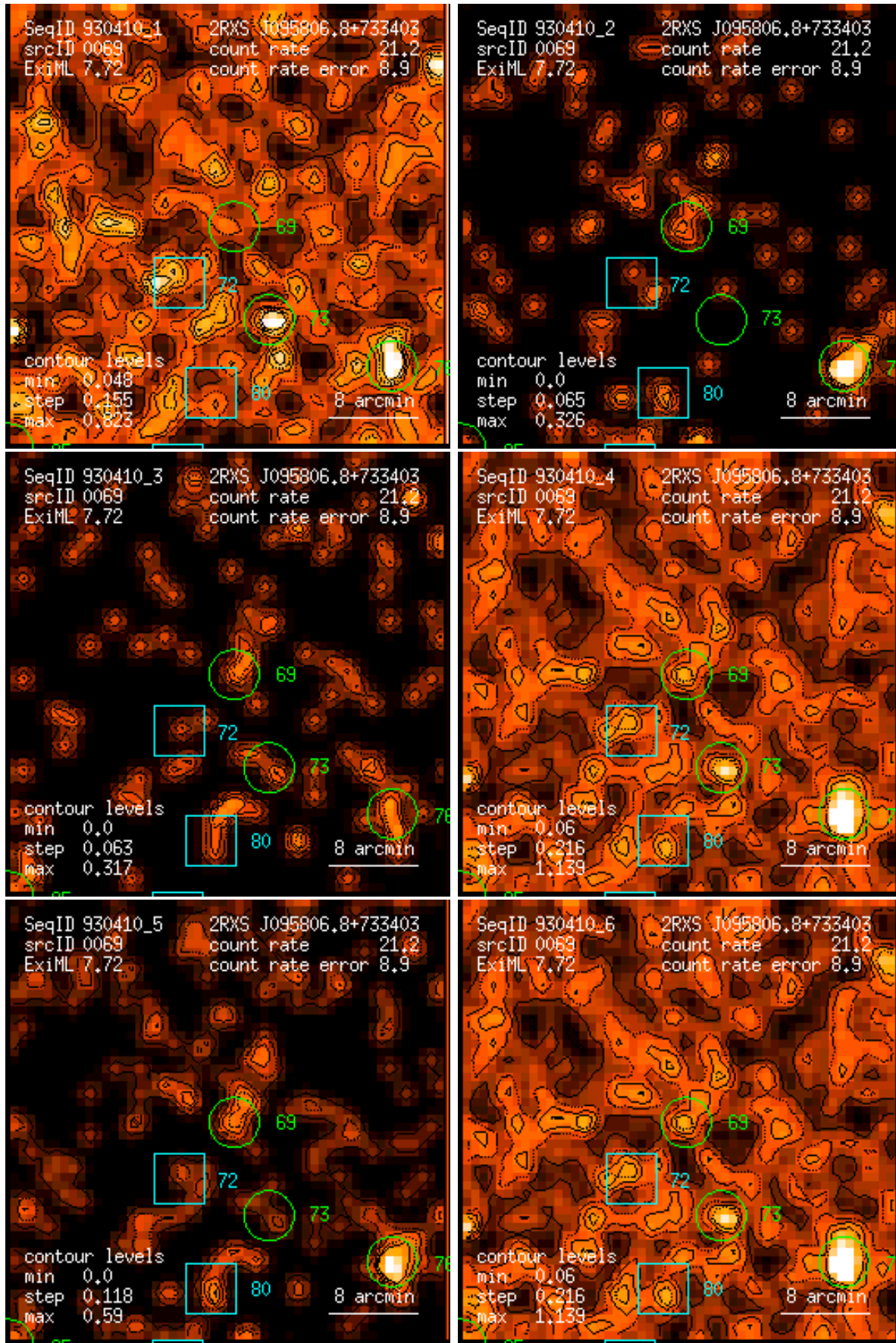
Figure 69: RASS 930410: detection 0069: band rate images, Gaussian filter: (1) PSPC channels 11 – 41, (2) 52 – 90, (3) 91 – 201, (4) 11 – 235, (5) 52 – 201, (6) 11 – 201. Broad band rates in counts/ks. Band rate contour levels in counts/ks/arcmin 2 .
