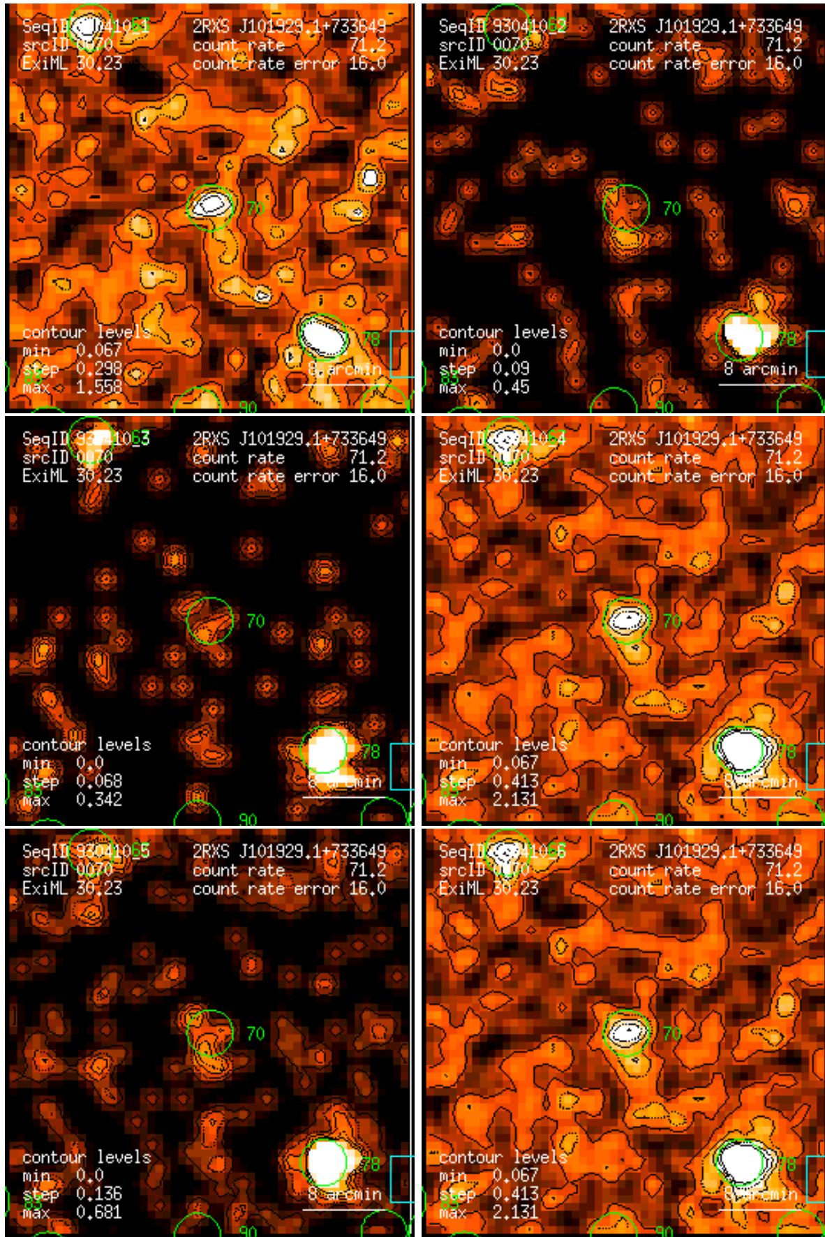
Figure 70: RASS 930410: detection 0070: band rate images, Gaussian filter: (1) PSPC channels 11 – 41, (2) 52 – 90, (3) 91 – 201, (4) 11 – 235, (5) 52 – 201, (6) 11 – 201. Broad band rates in counts/ks. Band rate contour levels in counts/ks/arcmin 2 .
