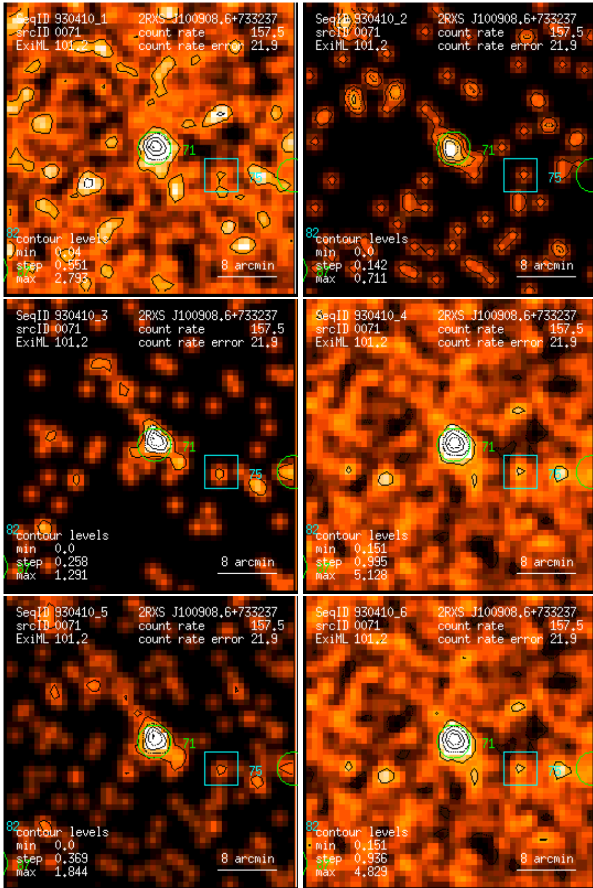
Figure 71: RASS 930410: detection 0071: band rate images, Gaussian filter: (1) PSPC channels 11 – 41, (2) 52 – 90, (3) 91 – 201, (4) 11 – 235, (5) 52 – 201, (6) 11 – 201. Broad band rates in counts/ks. Band rate contour levels in counts/ks/arcmin 2 .
