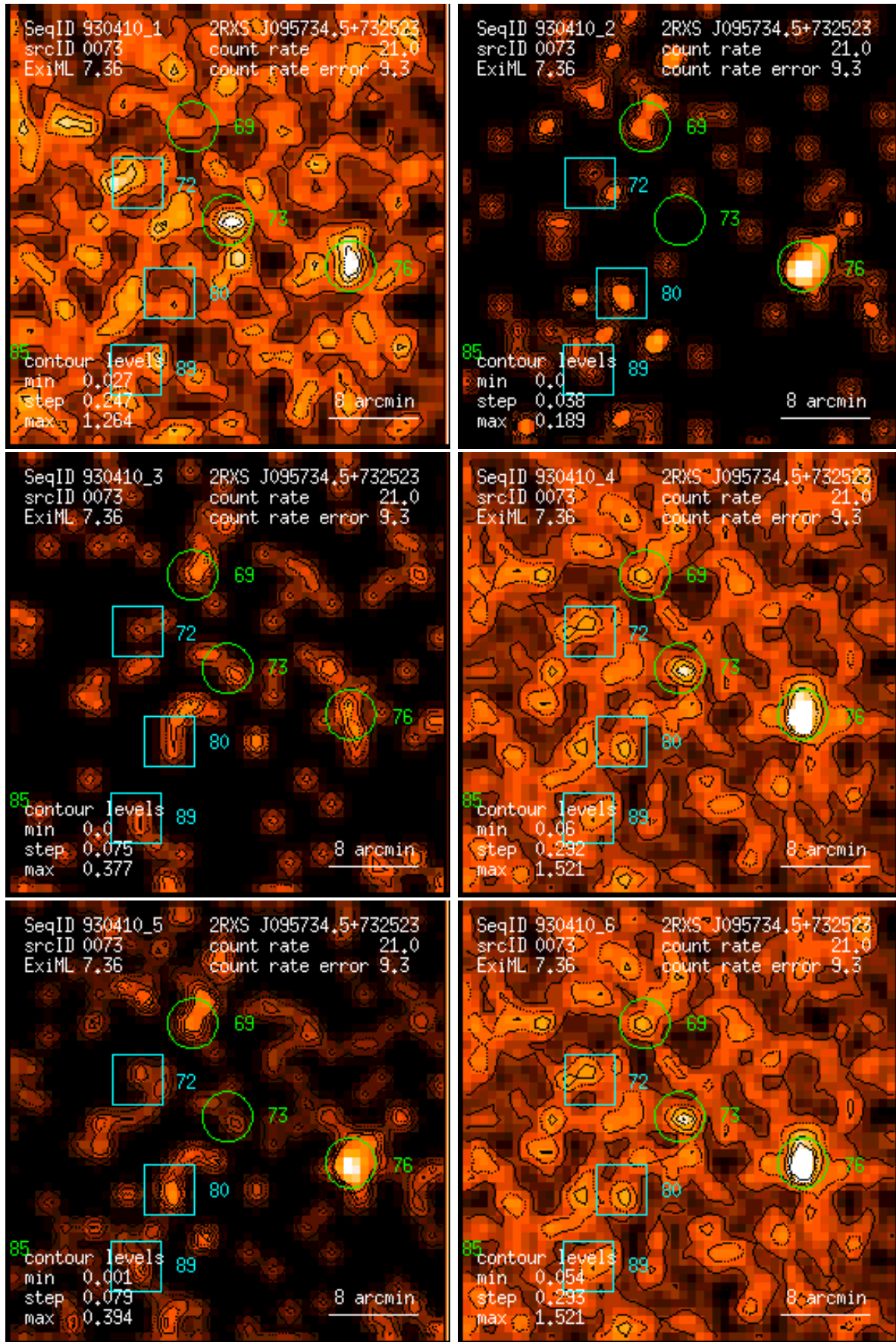
Figure 73: RASS 930410: detection 0073: band rate images, Gaussian filter: (1) PSPC channels 11 – 41, (2) 52 – 90, (3) 91 – 201, (4) 11 – 235, (5) 52 – 201, (6) 11 – 201. Broad band rates in counts/ks. Band rate contour levels in counts/ks/arcmin 2 .
