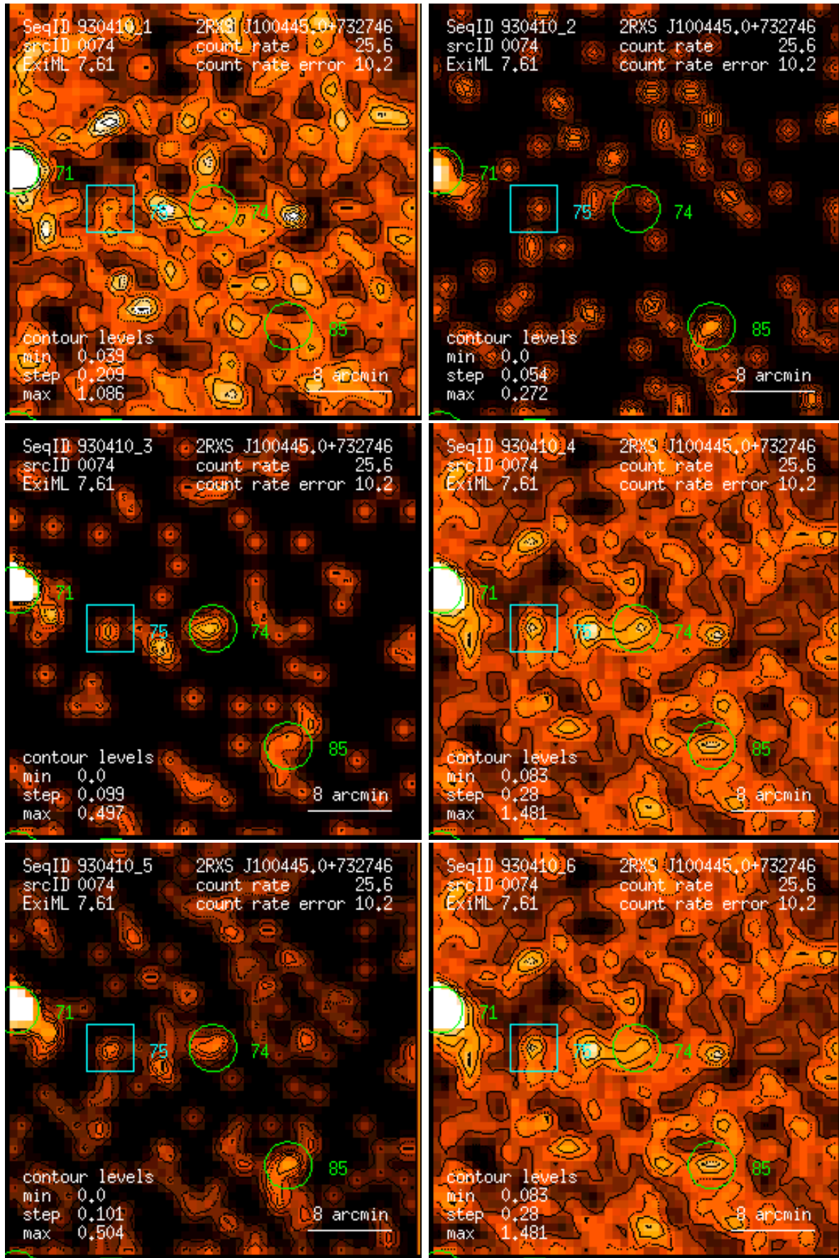
Figure 74: RASS 930410: detection 0074: band rate images, Gaussian filter: (1) PSPC channels 11 – 41, (2) 52 – 90, (3) 91 – 201, (4) 11 – 235, (5) 52 – 201, (6) 11 – 201. Broad band rates in counts/ks. Band rate contour levels in counts/ks/arcmin 2 .
