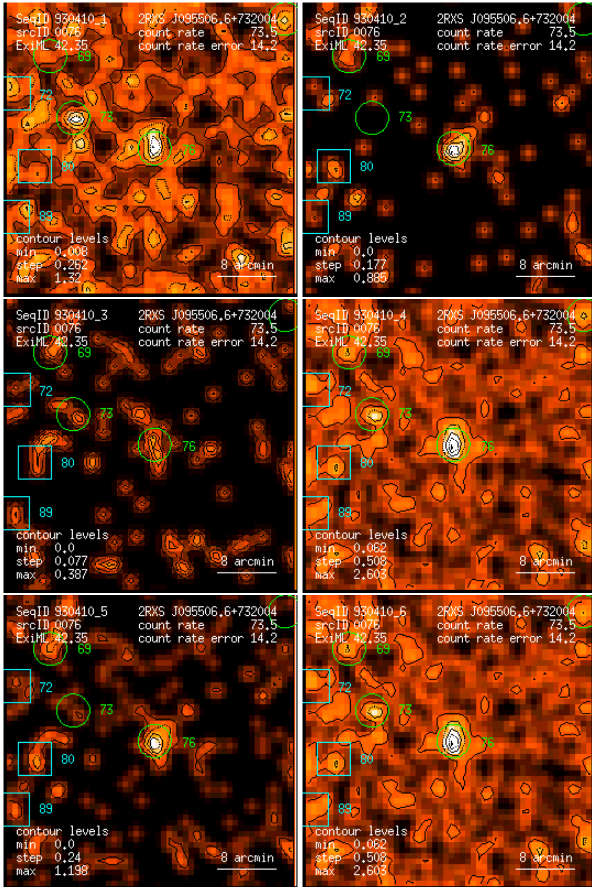
Figure 76: RASS 930410: detection 0076: band rate images, Gaussian filter: (1) PSPC channels 11 – 41, (2) 52 – 90, (3) 91 – 201, (4) 11 – 235, (5) 52 – 201, (6) 11 – 201. Broad band rates in counts/ks. Band rate contour levels in counts/ks/arcmin 2 .
