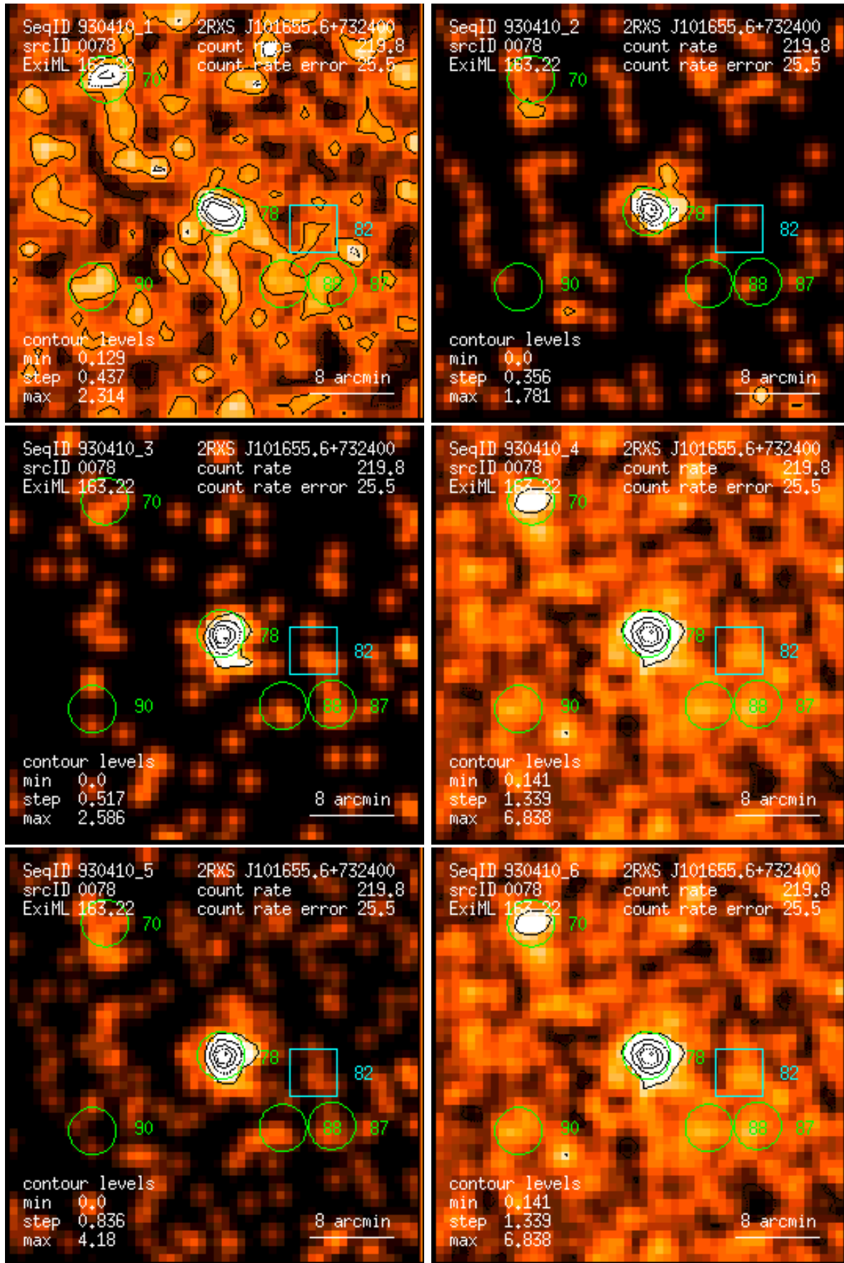
Figure 78: RASS 930410: detection 0078: band rate images, Gaussian filter: (1) PSPC channels 11 – 41, (2) 52 – 90, (3) 91 – 201, (4) 11 – 235, (5) 52 – 201, (6) 11 – 201. Broad band rates in counts/ks. Band rate contour levels in counts/ks/arcmin 2 .
