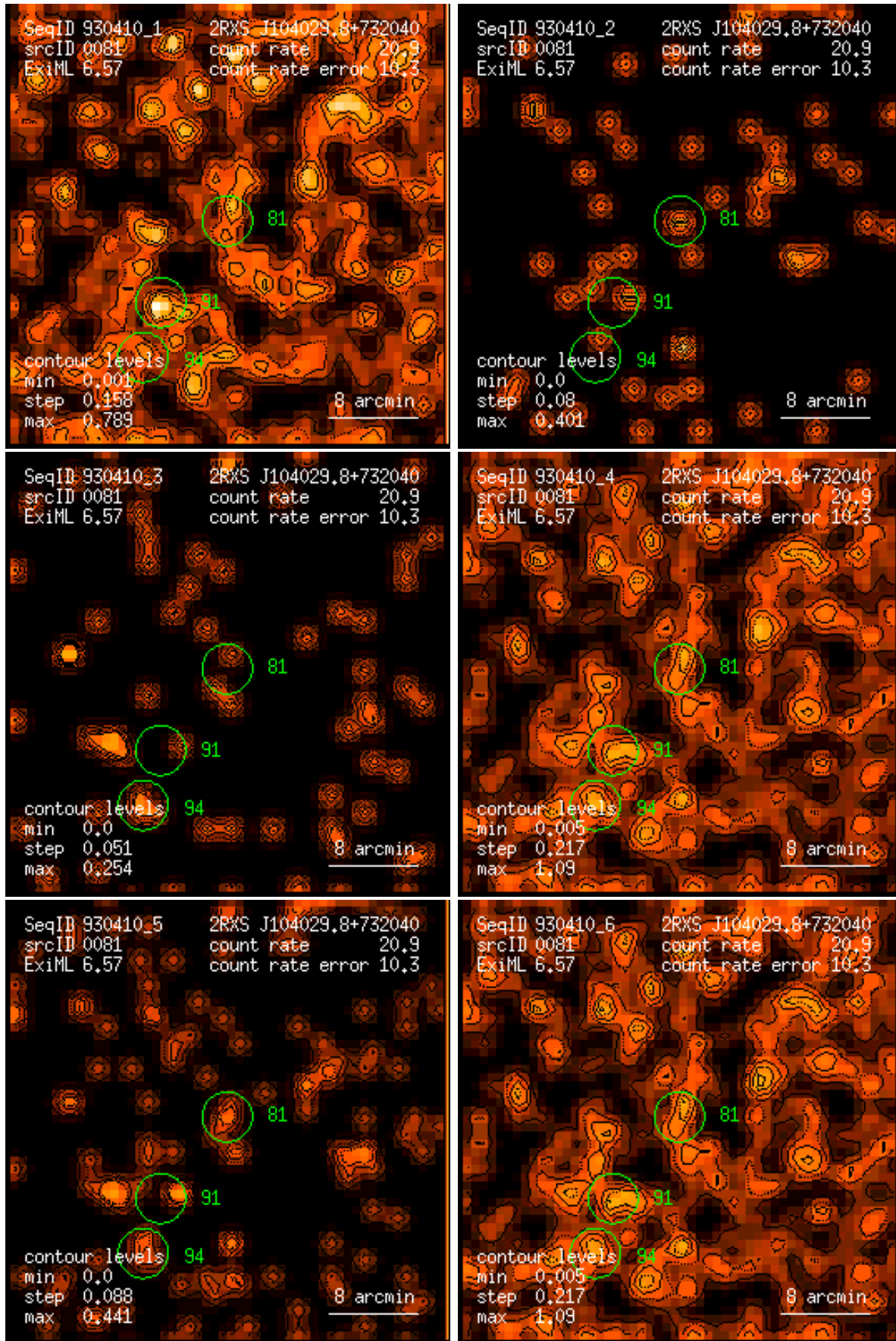
Figure 81: RASS 930410: detection 0081: band rate images, Gaussian filter: (1) PSPC channels 11 – 41, (2) 52 – 90, (3) 91 – 201, (4) 11 – 235, (5) 52 – 201, (6) 11 – 201. Broad band rates in counts/ks. Band rate contour levels in counts/ks/arcmin 2 .
