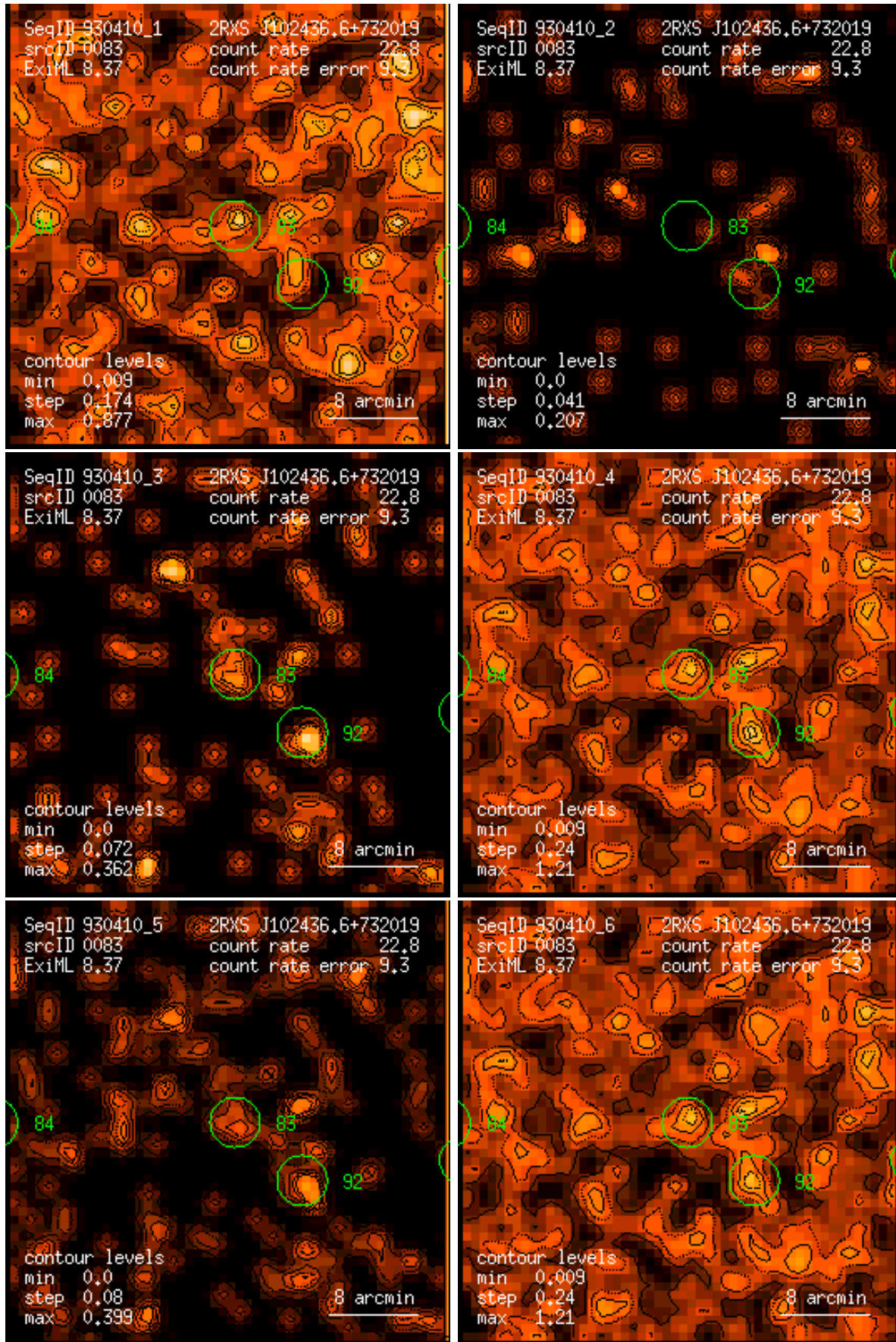
Figure 83: RASS 930410: detection 0083: band rate images, Gaussian filter: (1) PSPC channels 11 – 41, (2) 52 – 90, (3) 91 – 201, (4) 11 – 235, (5) 52 – 201, (6) 11 – 201. Broad band rates in counts/ks. Band rate contour levels in counts/ks/arcmin 2 .
